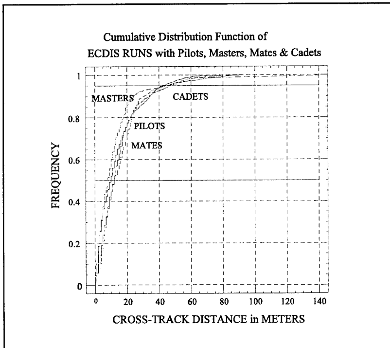
FIGURE 2 - ECDIS RUNS
