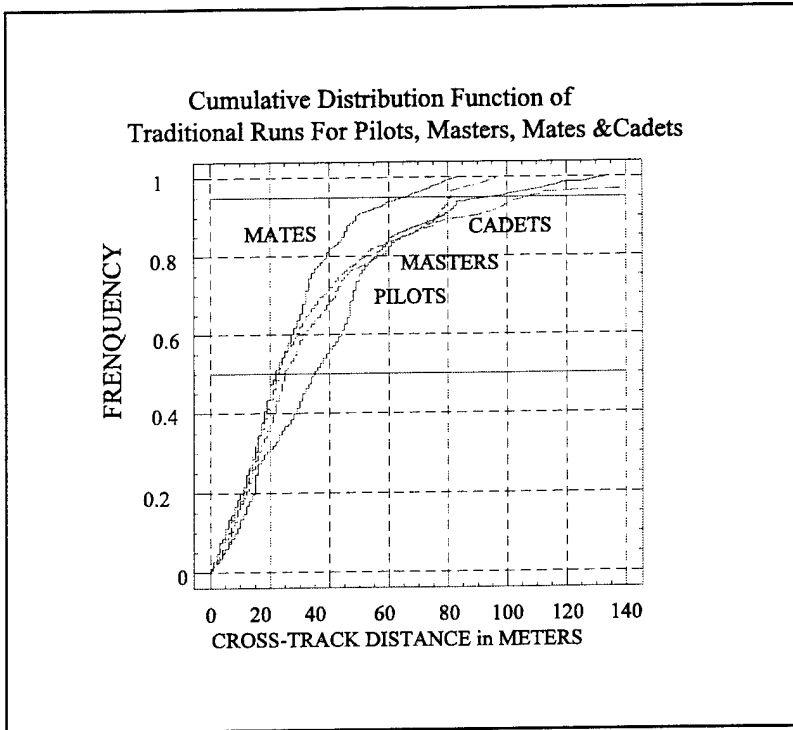
FIGURE 3 - TRADITIONAL RUNS
