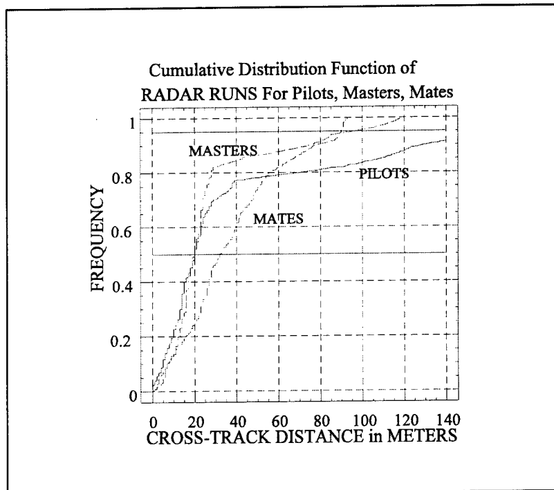
FIGURE 4 - RADAR RUNS
