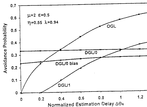
Fig. 6. The effect of estimation delay on the probability of interception avoidance.
