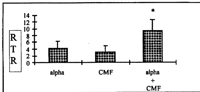
Figure : Relative transformation rate (RTR) of rat epithelial tracheal cells after \alpha -irradiation and/or exposure to combined magnetic fields (CMF). * = p < 0.05 vs control (U of Mann and Whitney).
