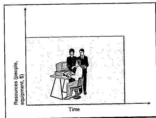
Figure 4. Time Box
