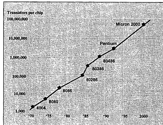
Figure 3. Moore's Law
