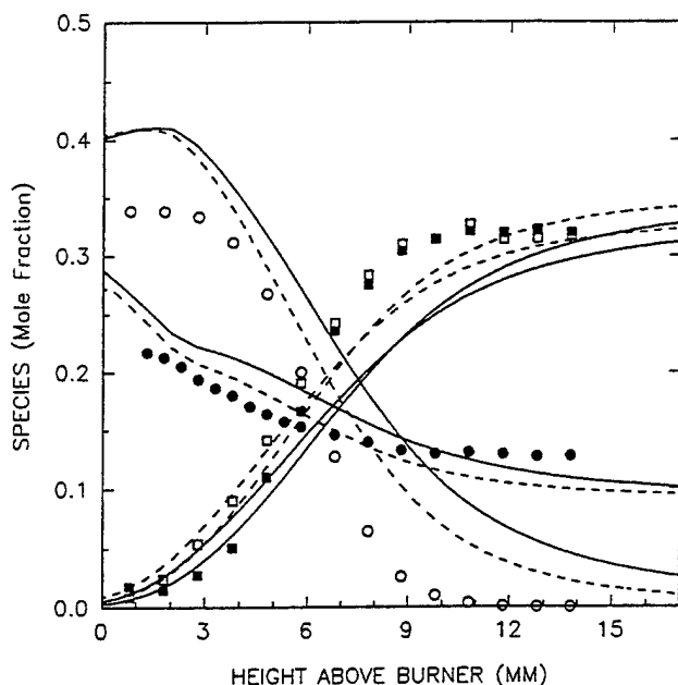
Figure 3. Calculated (—) and experimental \text{H}_2 (●), \text{N}_2\text{O} (○), \text{H}_2\text{O} (□), and \text{N}_2 (■) species profiles for a 30-torr \text{H}_2/\text{N}_2\text{O}/\text{Ar} flame doped with 4% \text{NH}_3 . The dashed curves are calculated profiles generated by increasing the temperature profile by a factor of 1.05, the experimental uncertainty.
