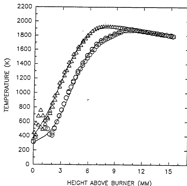
Figure 1. Temperature profiles of a neat ( \Delta ) and 4% \text{NH}_3 -doped ( \circ ), 30-torr \text{H}_2/\text{N}_2\text{O}/\text{Ar} flame. The solid line is a best fit of the data using a sigmoid-type function.
