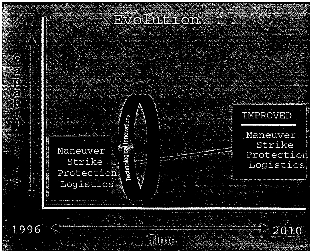
Figure 4. Evolutionary Trend
