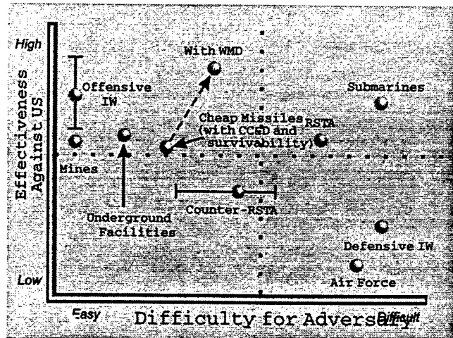
Figure 3. Asymmetric Counters
