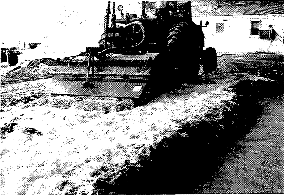
Figure 27. Mixing fibers into sand using rotary mixer
