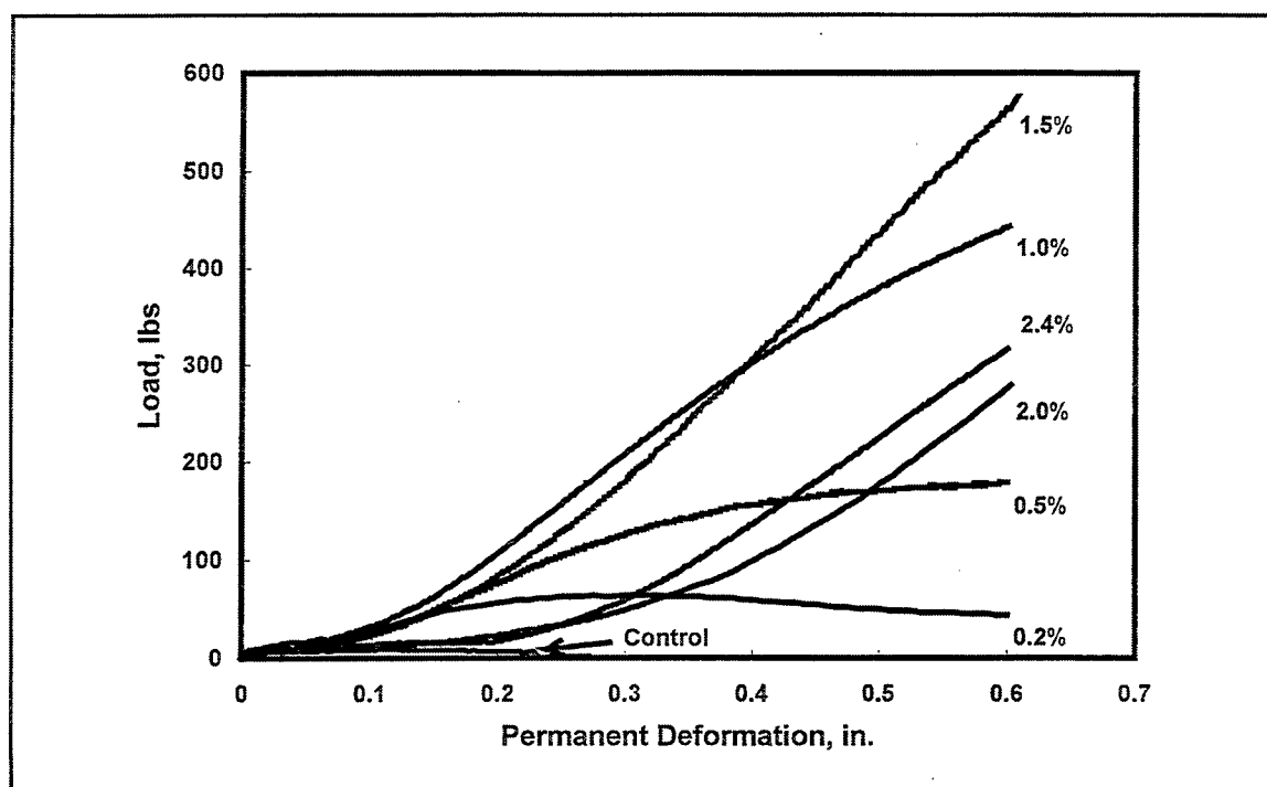
Figure 14. Relationship between percent of fiber and permanent deformation
