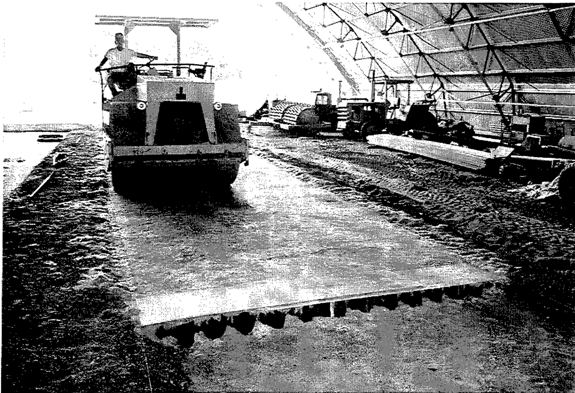
Figure 31. Compacting sand-fiber mixture into sand grid cells
