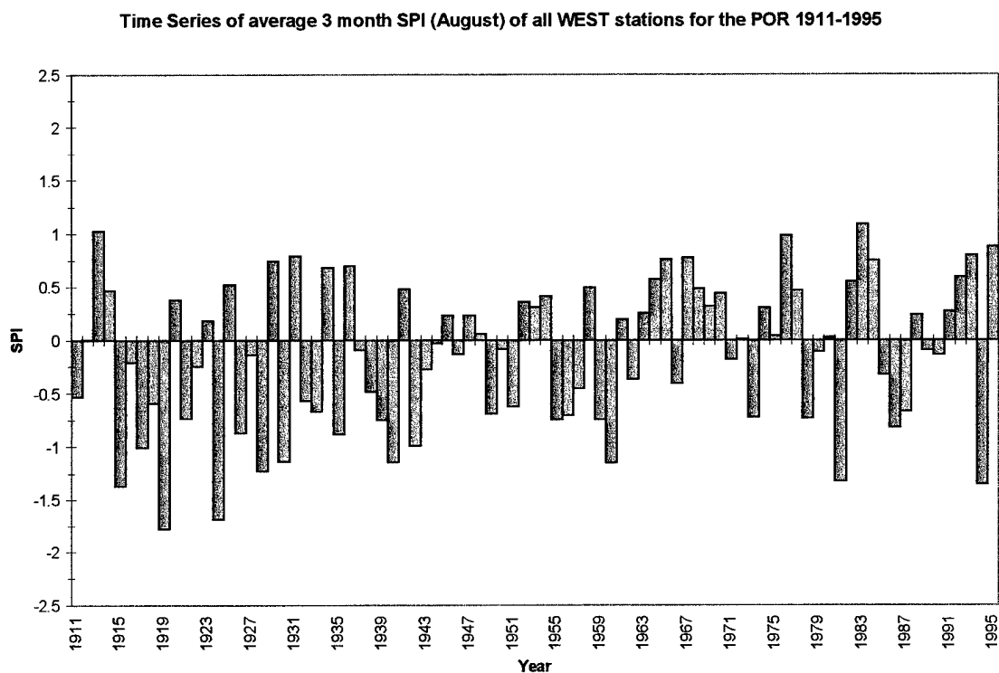
Fig 4.23(C) Time series of average 3 month SPI for August (summer) of all West stations for the period January, 1911 through December, 1995.
