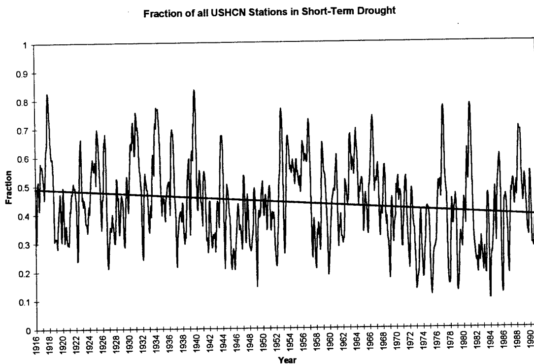
Fig 4.12 (B) Time series of the fraction of USHCN stations in short-term drought (3 month SPI) for the period Jan 1916 thru Dec 1990 with trend line.
