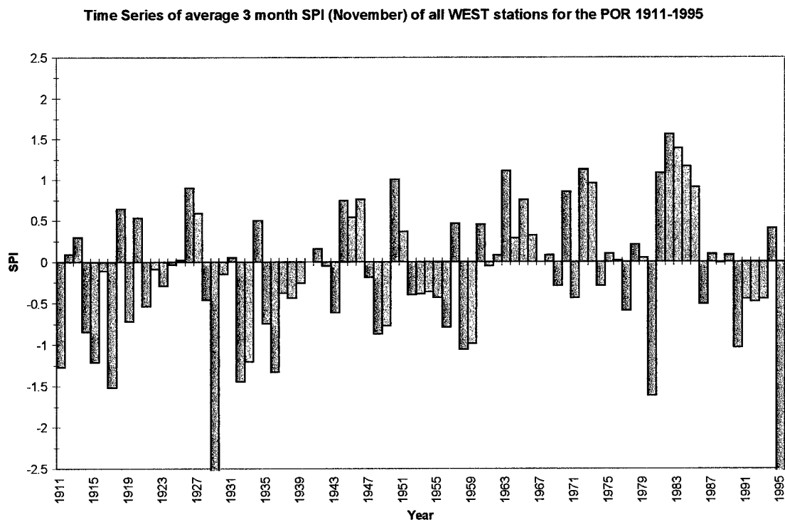
Fig 4.23(D) Time series of average 3 month SPI for November (autumn) of all West stations for the period January, 1911 through December, 1995.
