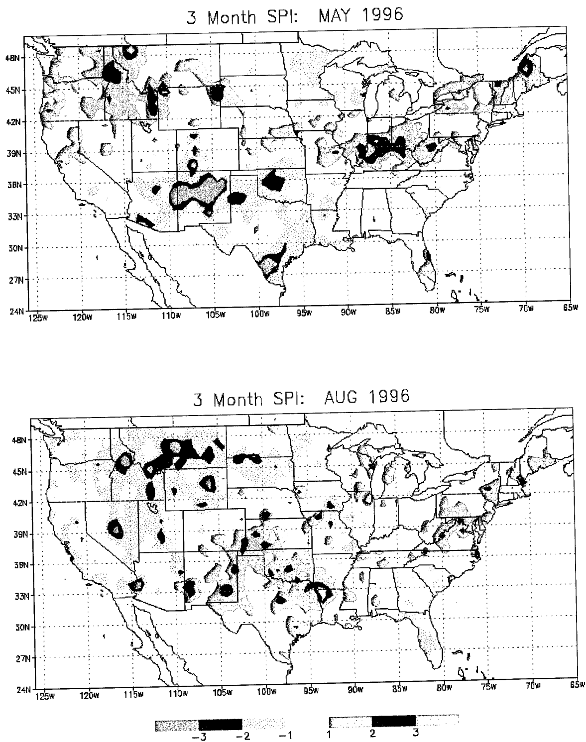
Fig 3.5 Comparison of spring drought of 1996 and summer wet period of 1996 in the Southern Plains and Southwest.
