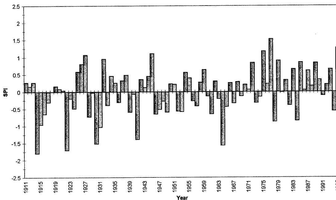
Fig 4.30(D) Time series of average 3 month SPI for November (autumn) of all Northeast stations for the period January, 1911 through December, 1995.
