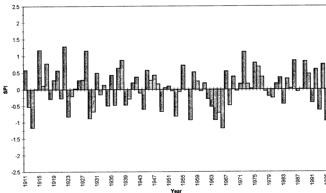
Fig 4.30(C) Time series of average 3 month SPI for August (summer) of all Northeast stations for the period January, 1911 through December, 1995.
