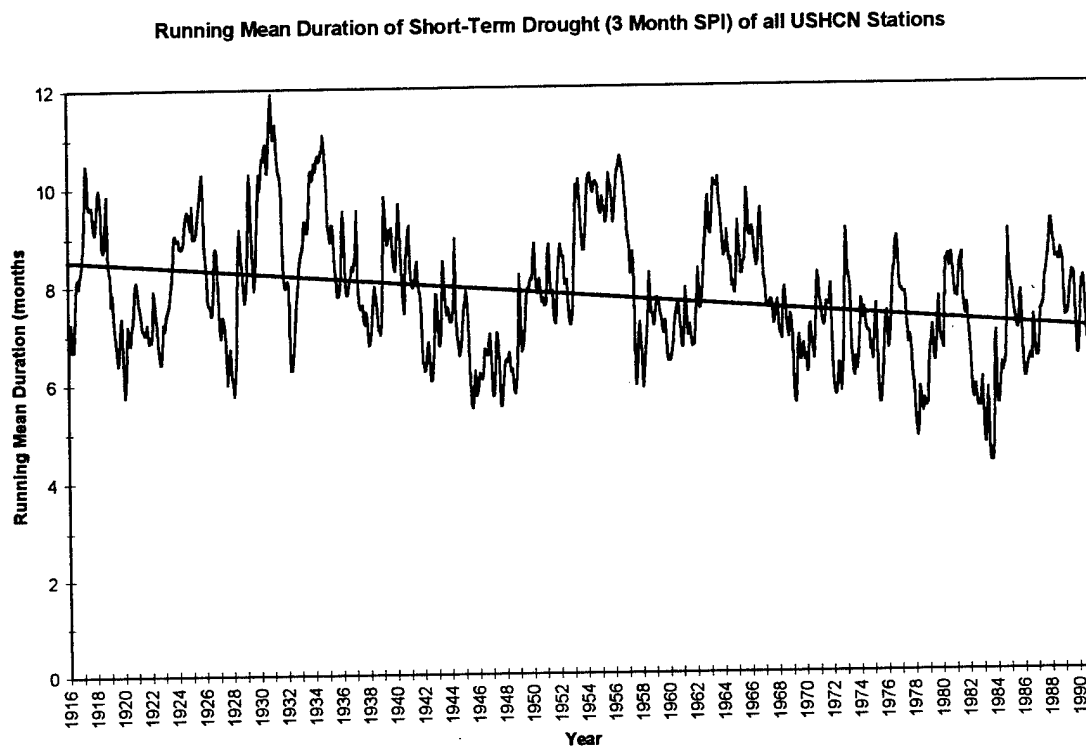
Fig 4.12 (A) Running mean duration of short-term drought (3 month SPI) of all USHCN stations for the period Jan 1916 thru Dec 1990 with trend line.
