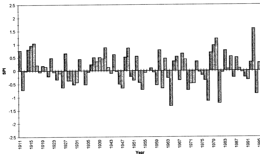
Fig 4.26(A) Time series of average 3 month SPI for February (winter) of all Southwest stations for the period January, 1911 through December, 1995.
