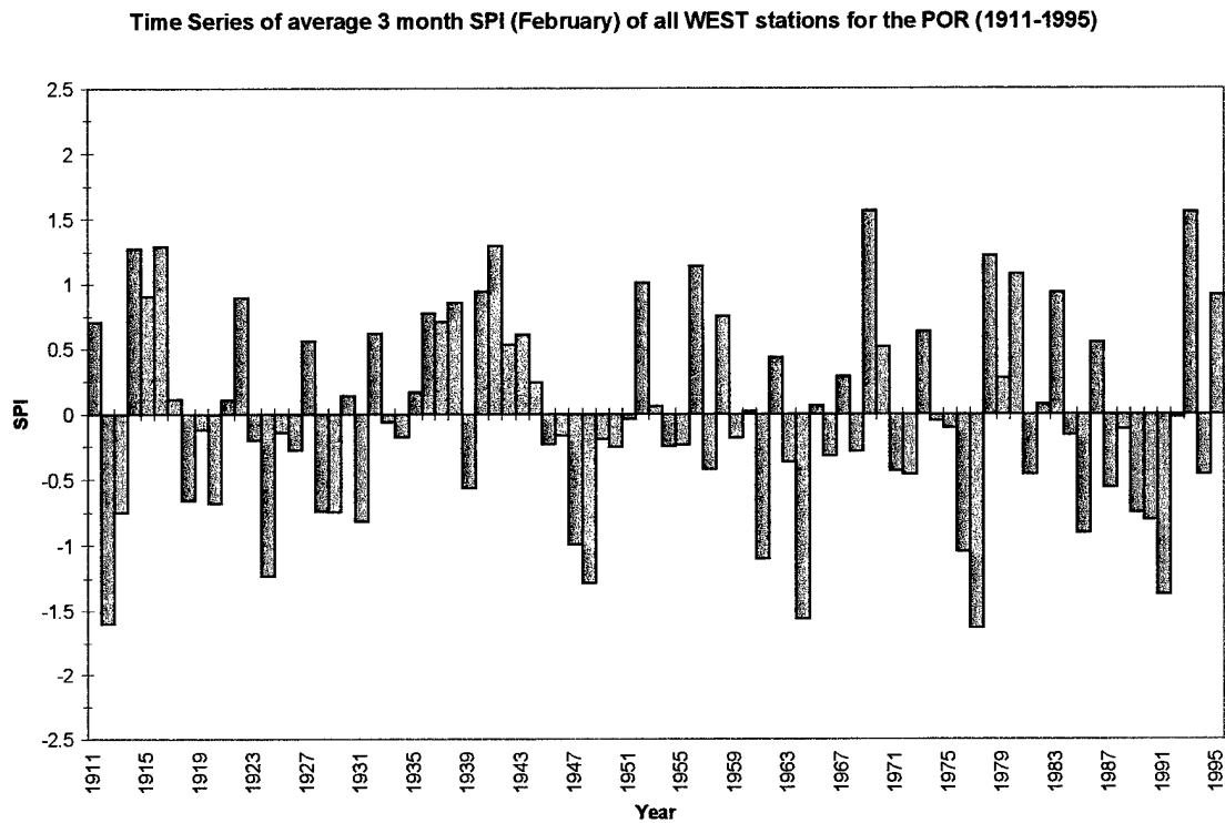
Fig 4.23(A) Time series of average 3 month SPI for February (winter) of all West stations for the period January, 1911 through December, 1995.
