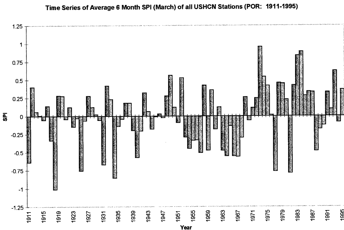
Fig 4.14 (B) Time series of average 6 month SPI for March (fall and winter) of all USHCN stations for the period January, 1911 through December, 1995.
