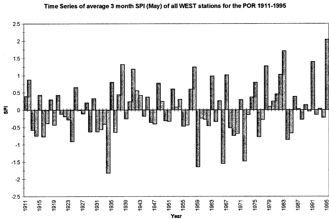
Fig 4.23(B) Time series of average 3 month SPI for May (spring) of all West stations for the period January, 1911 through December, 1995.
