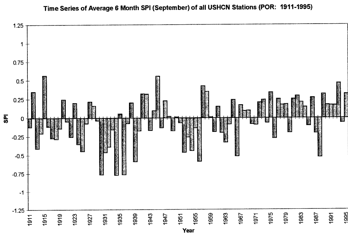
Fig 4.14 (A) Time series of average 6 month SPI for September (spring and summer) of all USHCN stations for the period January, 1911 through December, 1995.
