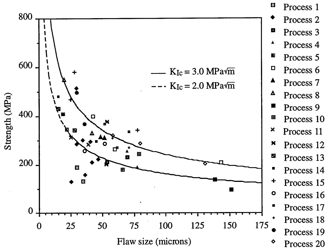
Fig. 5.11 Plot of strength vs. critical flaw size. Superimposed on the plot are the strengths predicted by eqn. 2.4 for a given critical flaw size assuming K_{Ic} values of 2.0 and 3.0 \text{MPa}\sqrt{\text{m}} .
