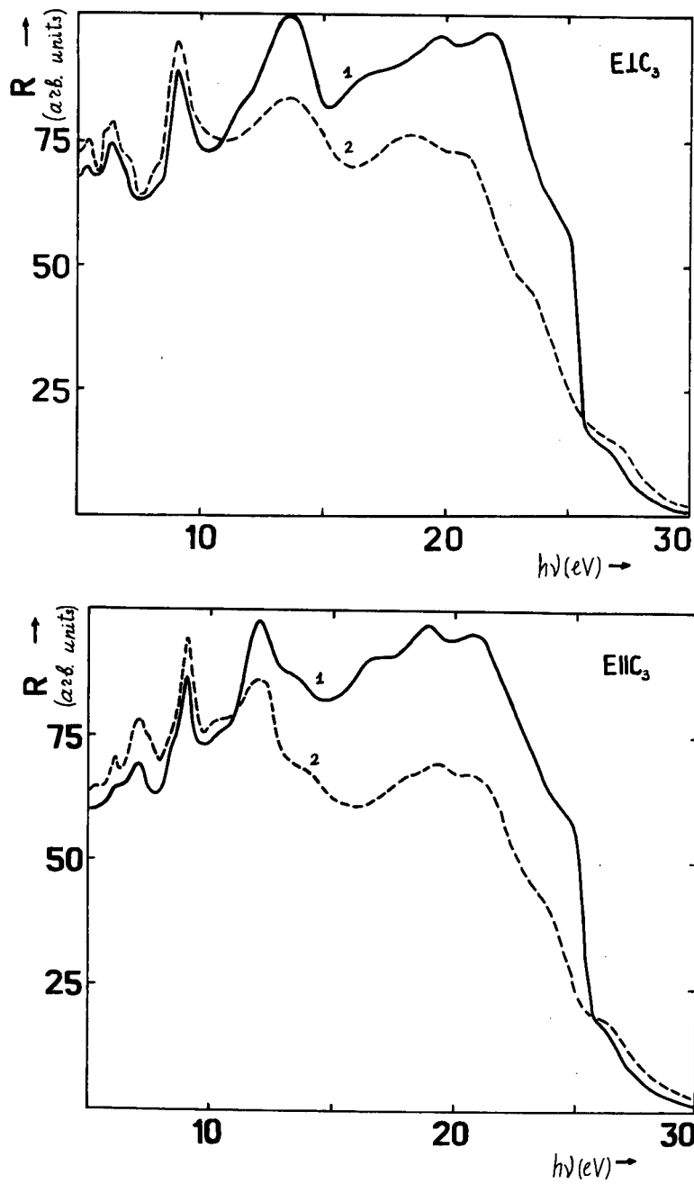
FIGURE 2 Reflection spectra of Verneil corundum monocrystals a. E \perp C_3 b. E \parallel C_3 curves : 1 - unirradiated crystal 2 - electron-irradiated with dose 3 \times 10^{17} \text{ e/cm}^2 .
