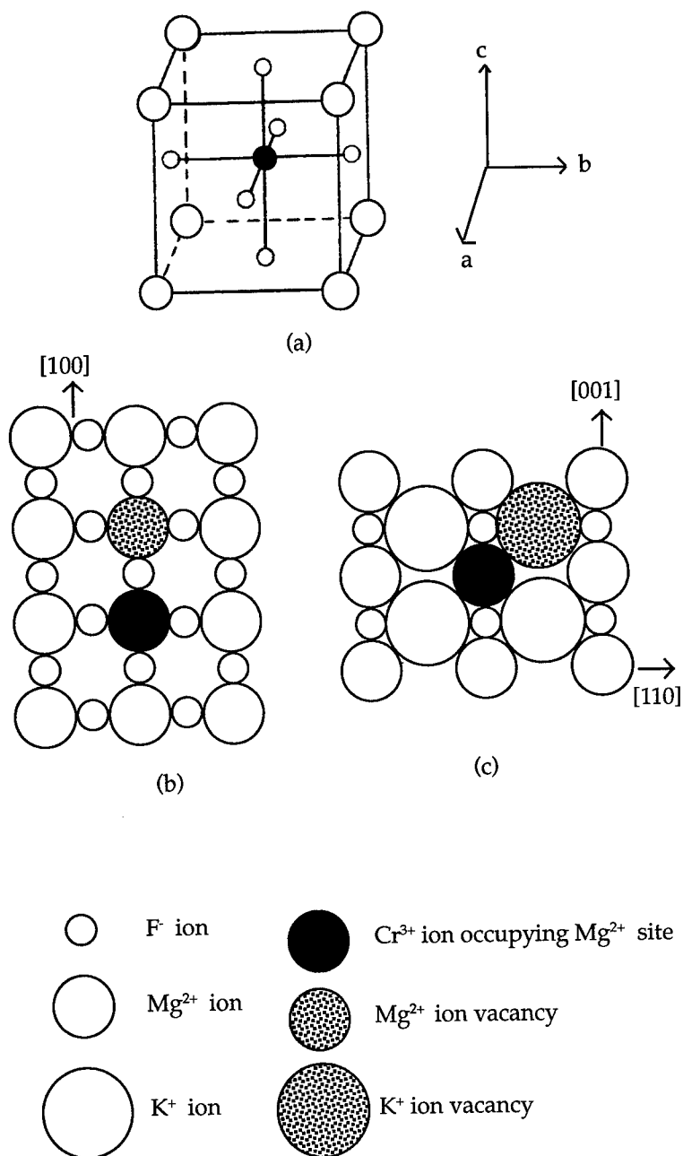
FIGURE 1 The KMgF_3 unit cell showing a Cr^{3+} ion substituted for a Mg^{2+} ion in an octahedral arrangement of six fluorine atoms. b A tetragonally distorted charge compensated Cr^{3+} site on the (001) plane. c A trigonally distorted charge compensated Cr^{3+} site on the (110) plane.
