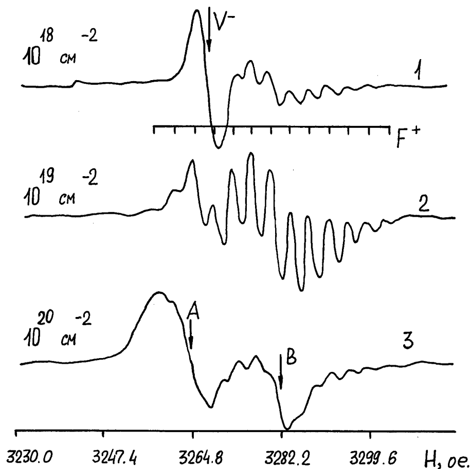
FIGURE 2 ESR spectra of \text{BeO} crystals irradiated with different neutron fluences.
