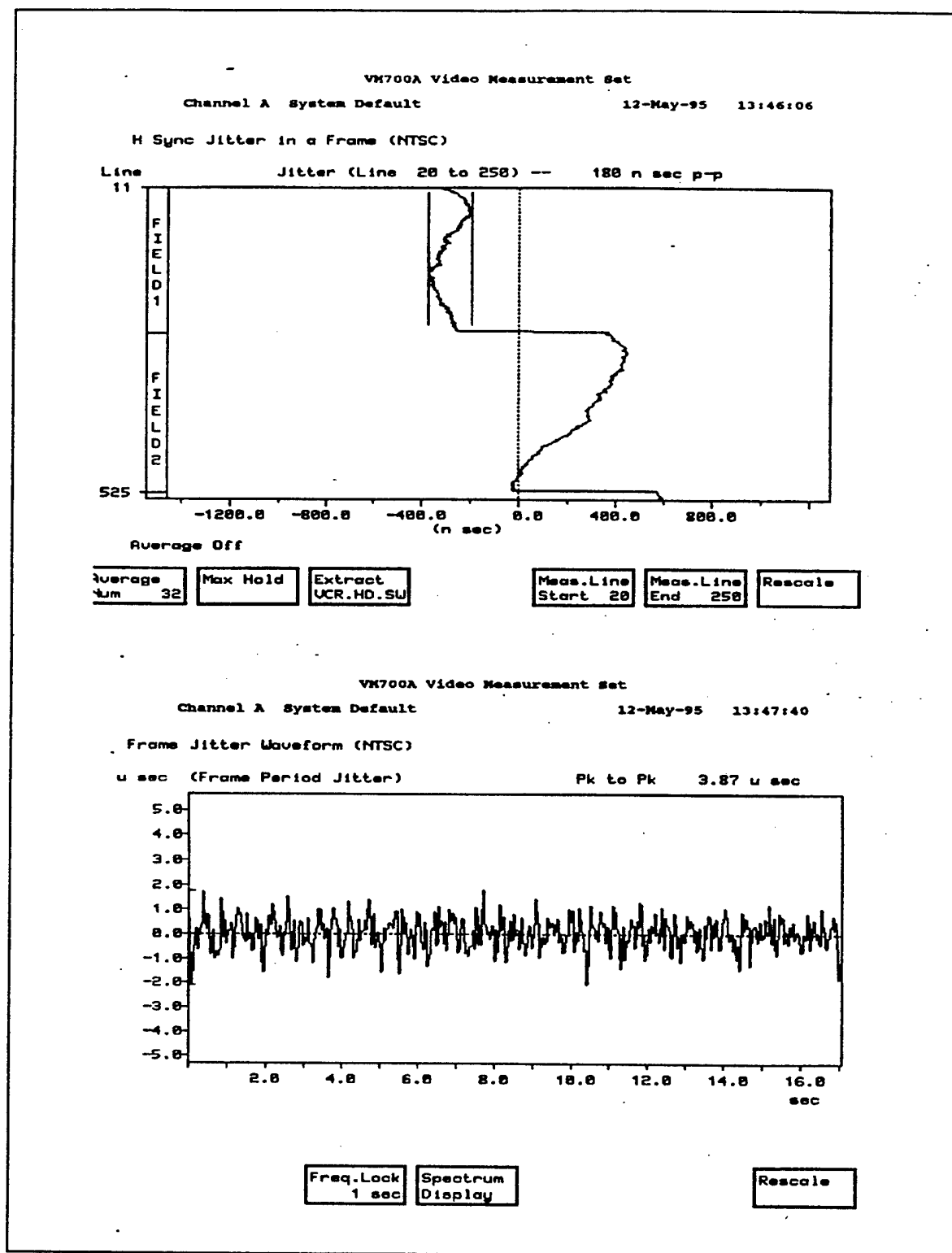
Figure B.2 Horizontal sync jitter of commercial quality VHS tape player
