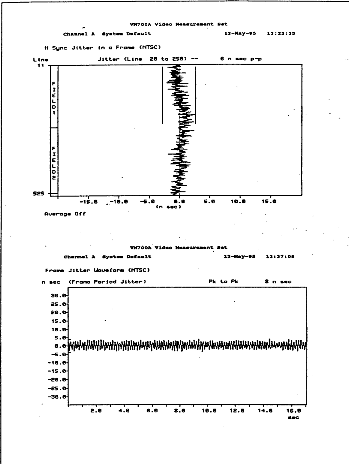
Figure B.3 Horizontal sync jitter of Betacam SP tape player
