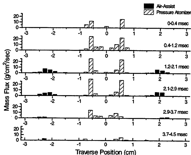
Figure 10: Mass Flux occurring at a Plane 1 cm Below the Injector for the Pressure Atomizer and Air Assist (Vol/Inj.=69 mm 3 )
