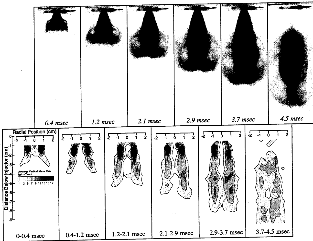
Figure 11: Spray Images and Mass Flux Contours for the High Pressure Atomizer ( \text{Vol/inj}=69 \text{ mm}^3 )
