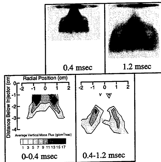
Figure 12: Spray Images and Mass Flux Contours for the High Pressure Atomizer ( \text{Vol/inj}=20 \text{ mm}^3 )
