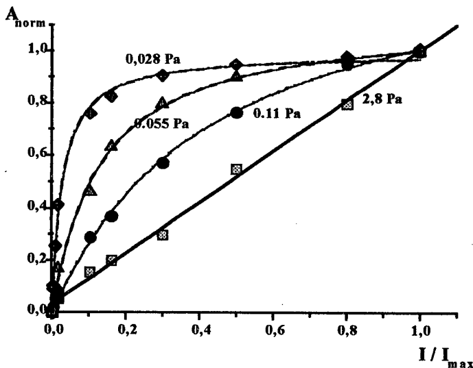
Fig. 2. The dependencies of photoadsorption initial rates A_{norm} on normalized light intensity ( I/I_{max} ) at several pressure for ZrO_2 - O_2 .
