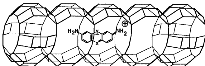
Figure 1: Schematic view of a dye molecule in the large channel of zeolite L.
