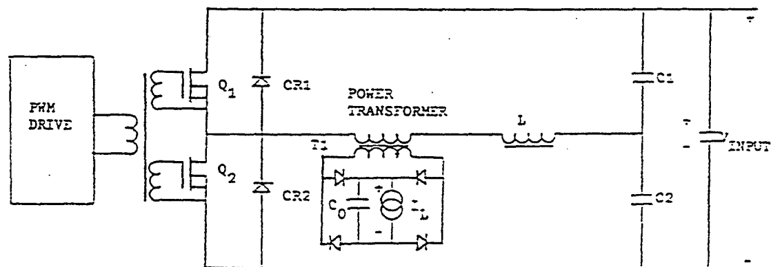
Figure 6.2-12 Circuit Application
