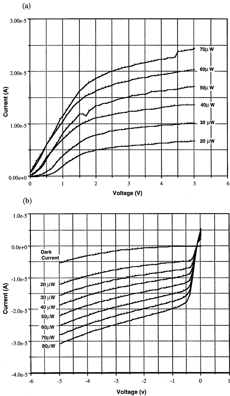
Figure 5-1. Current-voltage (IV) curves of a Si dual-metal MSM photodetector for a range of optical inputs. The plot labeled (a) shows the detector in the normal operating mode and in (b) the anode and cathode connections are swapped.
