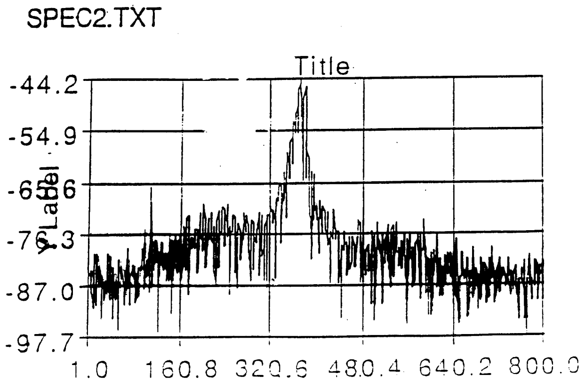
Figure 21. Frequency Noise Spectrum 8 th Harmonic
