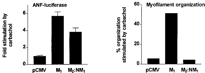
Fig. 4. Dissociation between the ability of the chimeric M 2 :NM 1 receptor to stimulate ANF-luciferase expression and induce myofilament organization. Myocytes were transfected with the indicated receptors cDNAs and either the ANF-luciferase reporter gene or RSV-luciferase. Following a 48 hr incubation in the absence or presence of carbachol, cells were either lysed and luciferase activity measured (left) or were fixed, stained and analyzed for myofilament organization (right) as described for Fig. 3.
