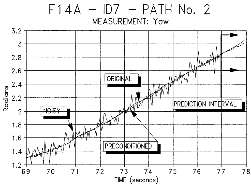
Figure 3.5 Trajectory Measurement Data: Yaw
