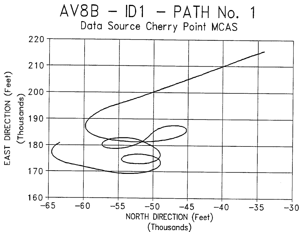
Figure 6.13 Plan View of Complete AV-8B Trajectory
