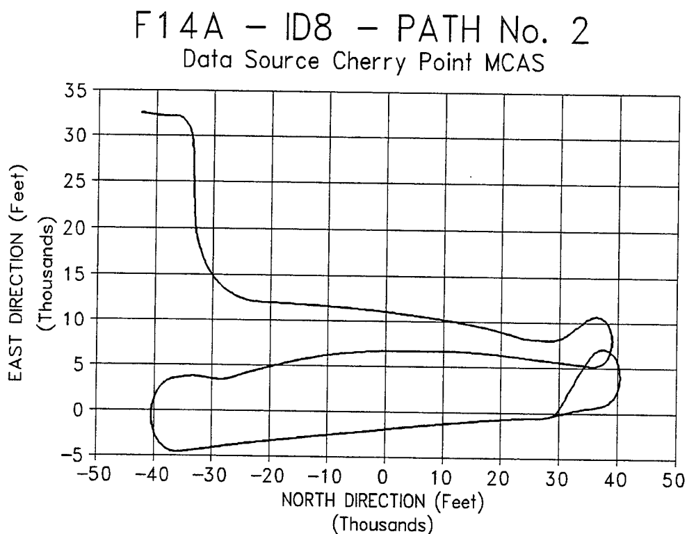
Figure 6.12 Plan View of Complete F-14A Trajectory
