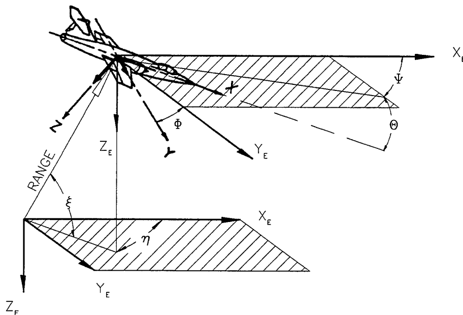
Figure 1.3 Measurement Geometry
