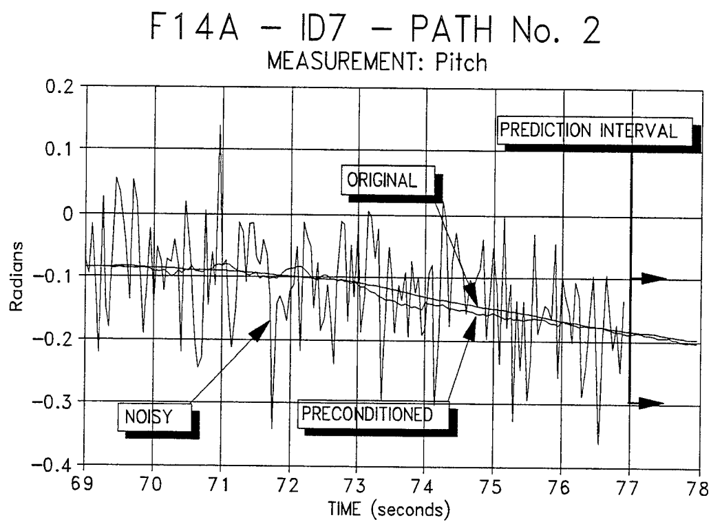
Figure 3.4 Trajectory Measurement Data: Pitch
