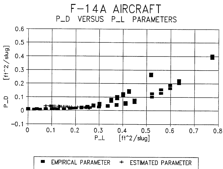
Figure 4.4 Empirical and Estimated F-14A Aircraft Parameters Correlation
