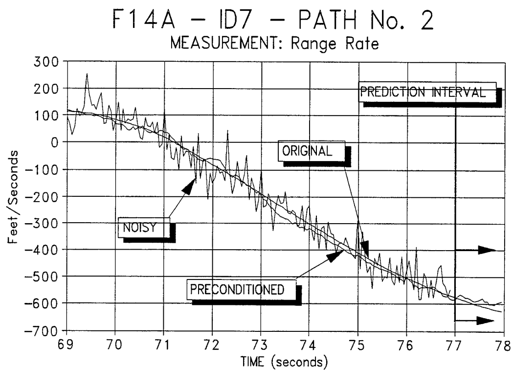
Figure 3.9 Trajectory Measurement Data: Range Rate
