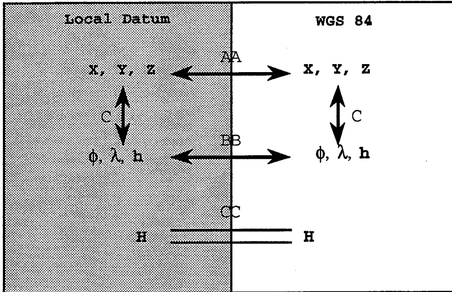
Figure 8.3. Datum shifts.
