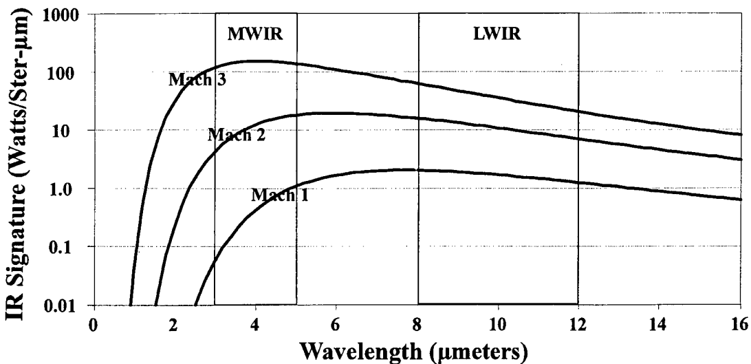
Figure 5. Target signature caused by aerodynamic heating for three target speeds
