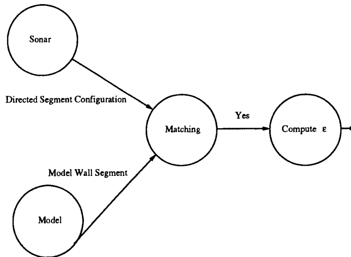
Figure 128. Matching algorithm
