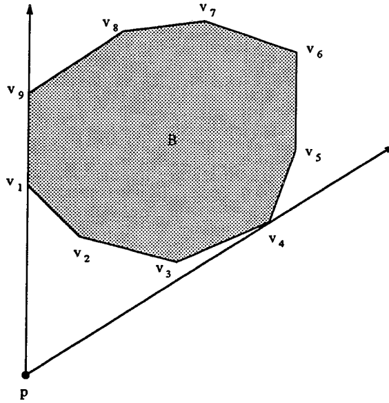
Figure 23. Visibility from point p to convex polygon B (II)
