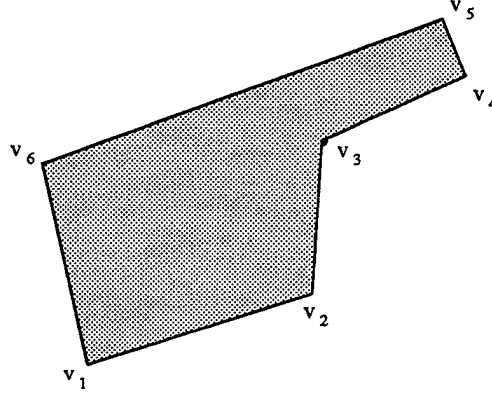
Figure 17. Concave polygon and its subpolygons (II)
