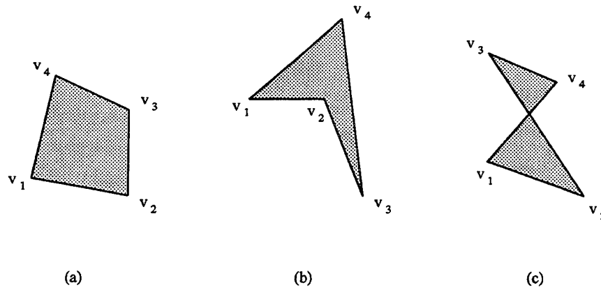
Figure 5. Simple and non-simple polygon (I)
