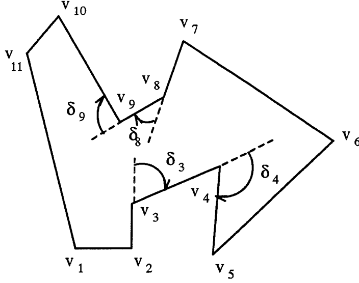
Figure 14. Concave polygon
