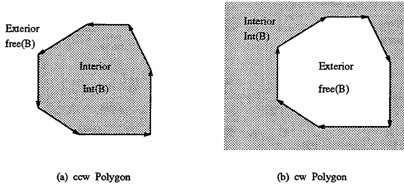
Figure 13. Interior and exterior of a simple polygon
