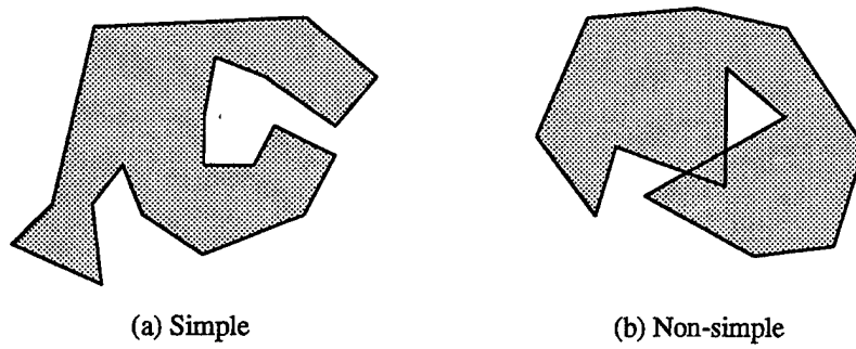
Figure 6. Simple and non-simple polygon (II)
