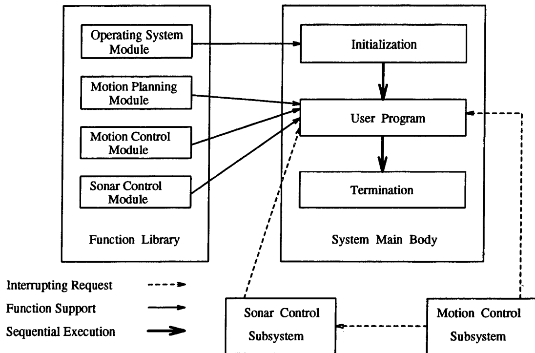
Figure 141. MML-11 software conceptual architecture
