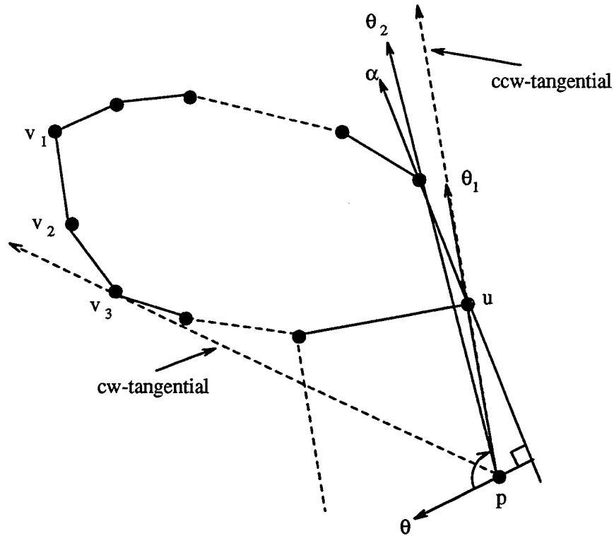
Figure 27. Correctness of image type algorithm
