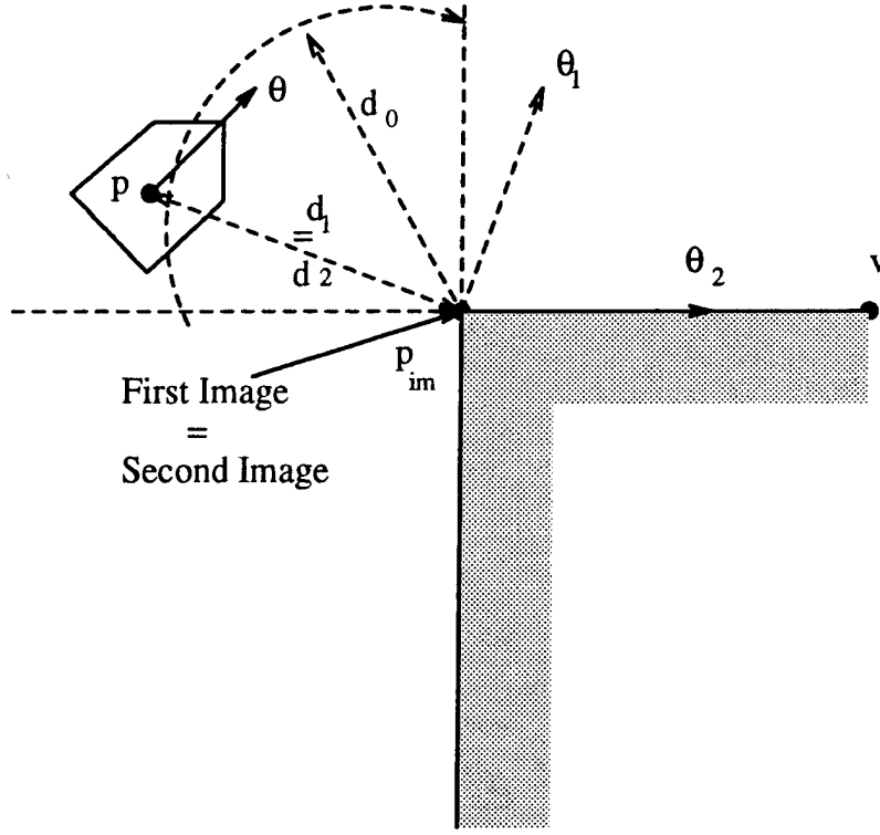
Figure 75. cw tracking of Vertex Tracking Mode
