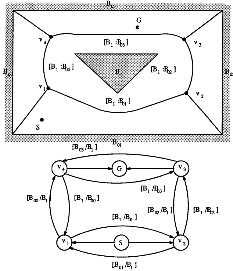
Figure 58. Solution of problem 3: world and augmented connectivity graph
