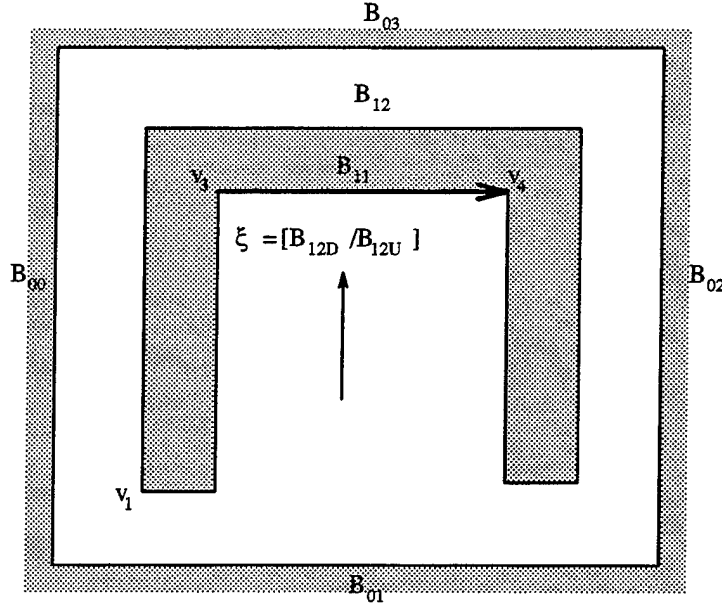
Figure 56. Solution of problem 2: up and down directed v-edges (I)
