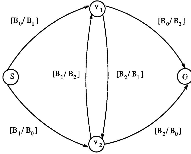
Figure 47. Augmented connectivity graph of a polygonal world (I)
