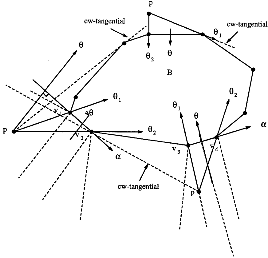
Figure 25. Image of point p lies on vertex v_i of convex polygon B
