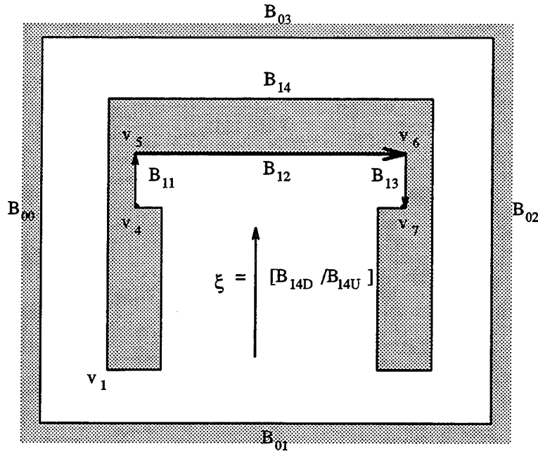
Figure 57. Solution of problem 2: up and down directed v-edges (II)
