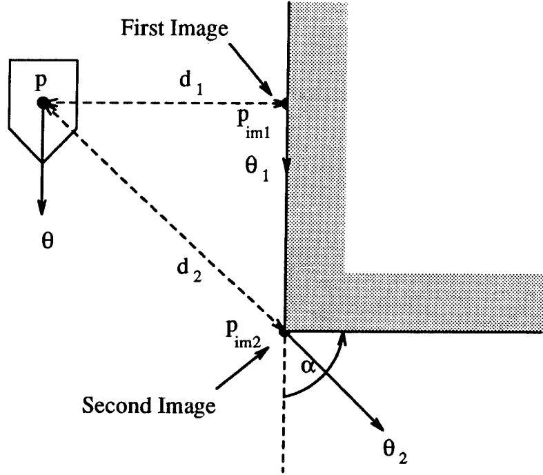
Figure 69. ccw tracking in Edge-Convex Vertex Tracking Mode
