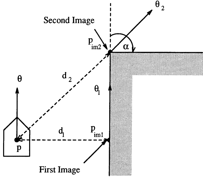
Figure 70. cw tracking in Edge-Convex Vertex Tracking Mode
