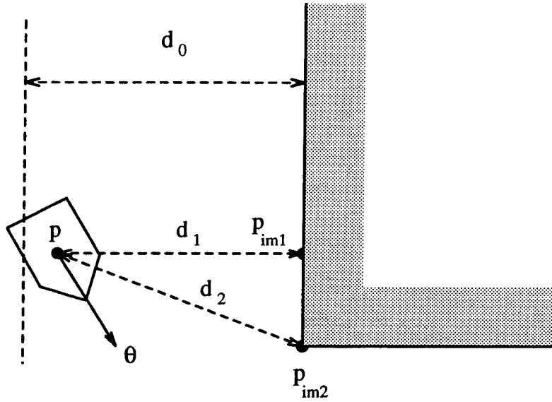
Figure 71. Calculate safety clearance function of ccw tracking
