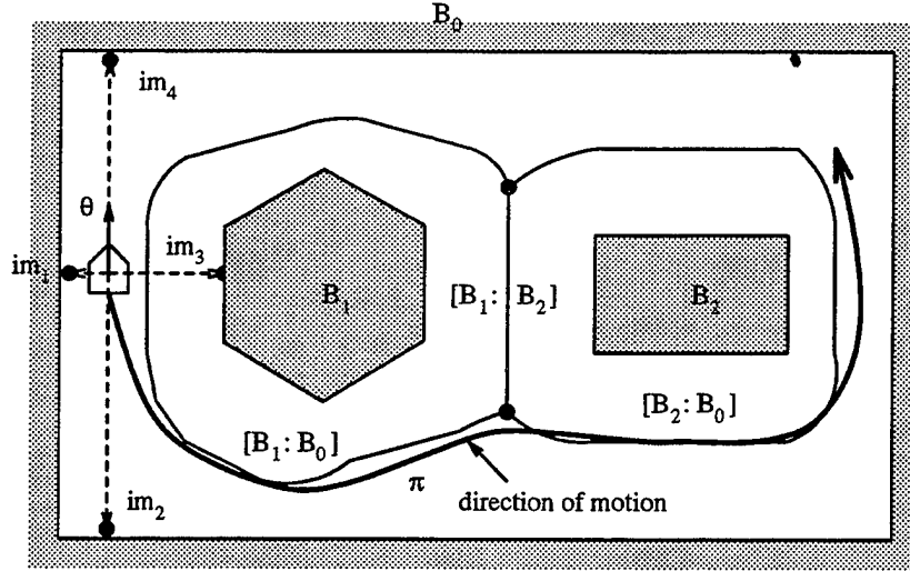
Figure 50. Problem 1: initial orientation of a vehicle is different from the direction of a motion
