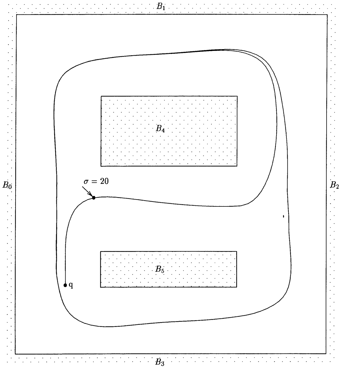
Figure 135: Yamabico-11 local motion planning and execution result (III)
