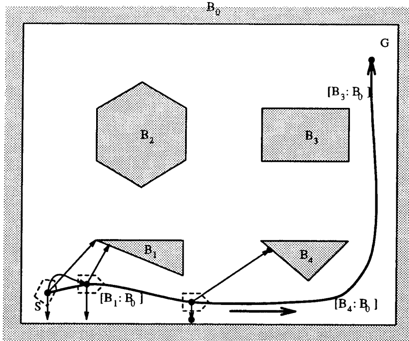
Figure 95. Directed v-edges sequence to local motion planning (no turn is required)
