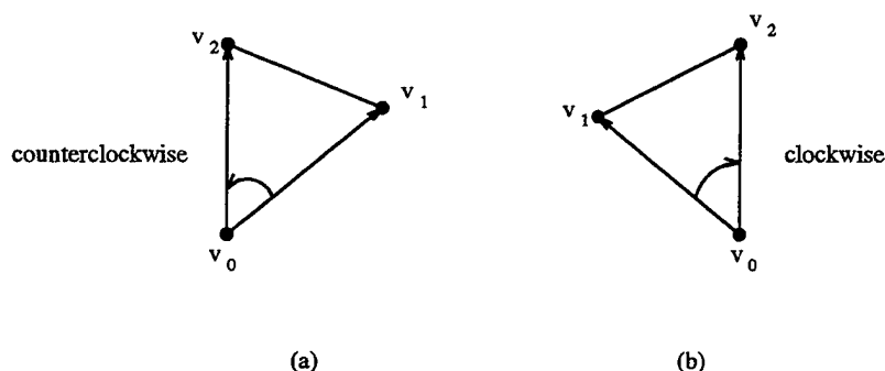
Figure 12. Using the cross product to determine how consecutive line segments \overline{v_0v_1} and \overline{v_1v_2} turn at a point v_1
