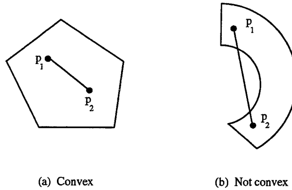
Figure 10. Convex set
