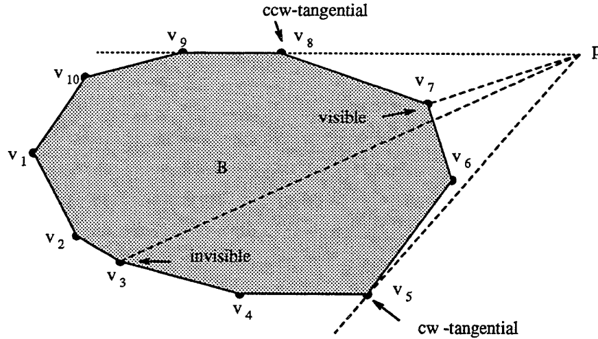
Figure 21. Visibility from point p to convex polygon B (I)
