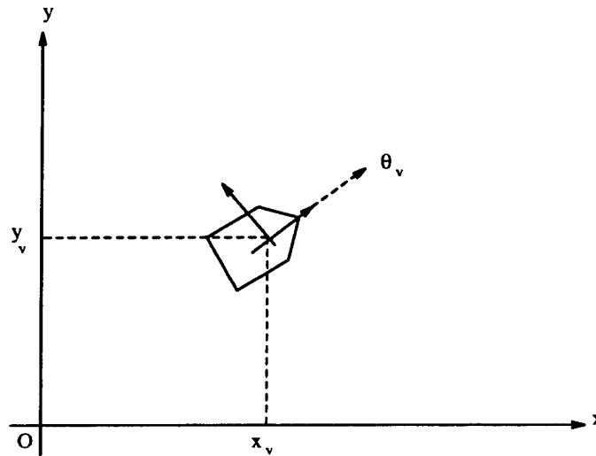
Figure 121. Positioning of rigid body robot as configuration
