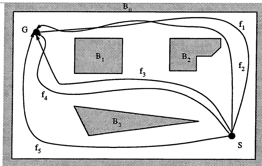
Figure 30. A world and paths
