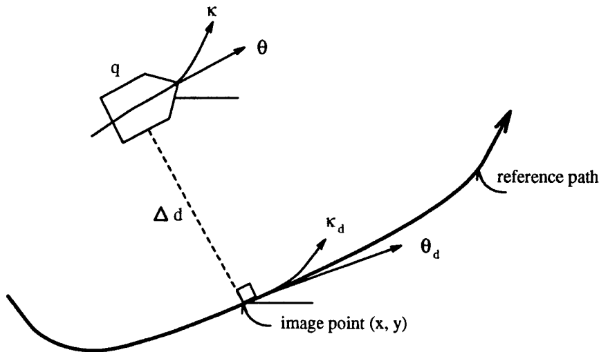
Figure 64. Geometrical concepts of steering function
