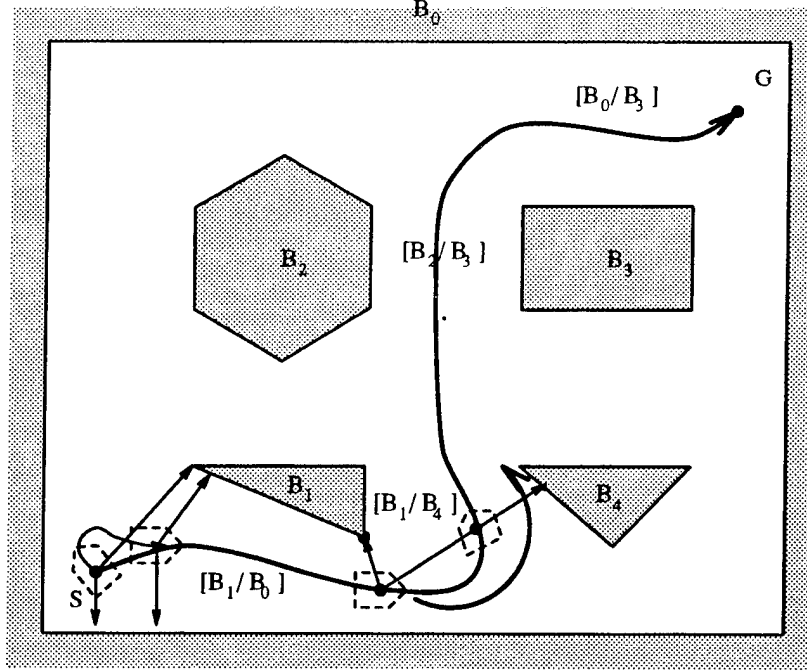
Figure 94. Directed v-edges sequence to local motion planning (left turn is required)
