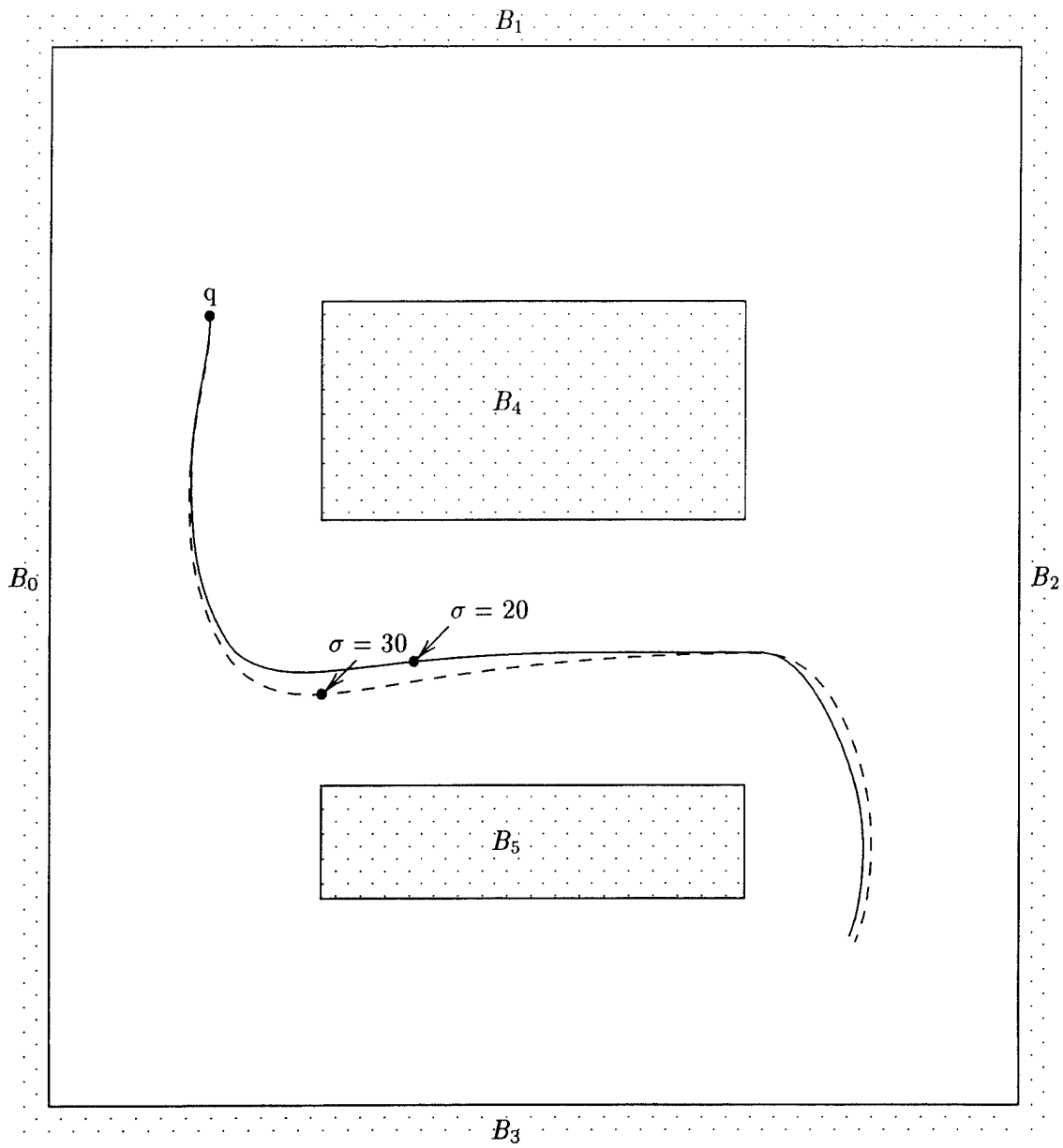
Figure 133: Yamabico-11 local motion planning and execution results (I)
