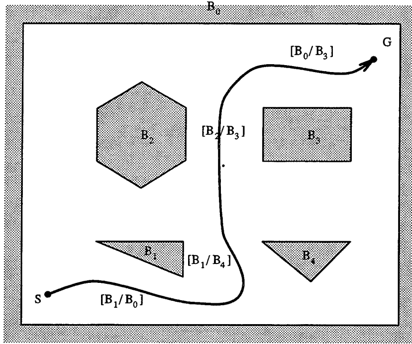
Figure 42. Directed v-edges sequence (I)
