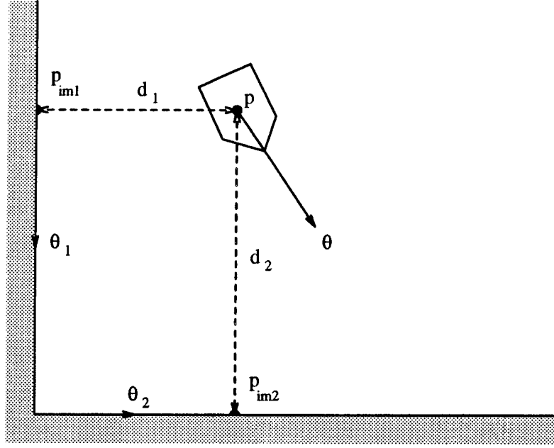
Figure 77. ccw tracking in Edge-Concave Vertex Tracking Mode
