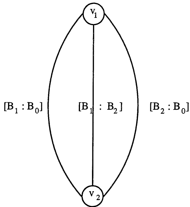
Figure 44. Basic connectivity graph of a polygonal world (I)
