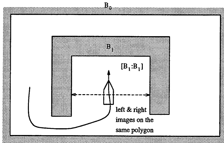
Figure 51. Problem 2: directed v-edge of a concave polygon
