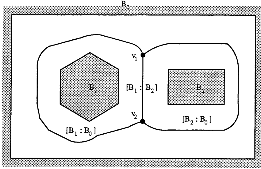
Figure 36. Voronoi diagram of polygonal world (I)
