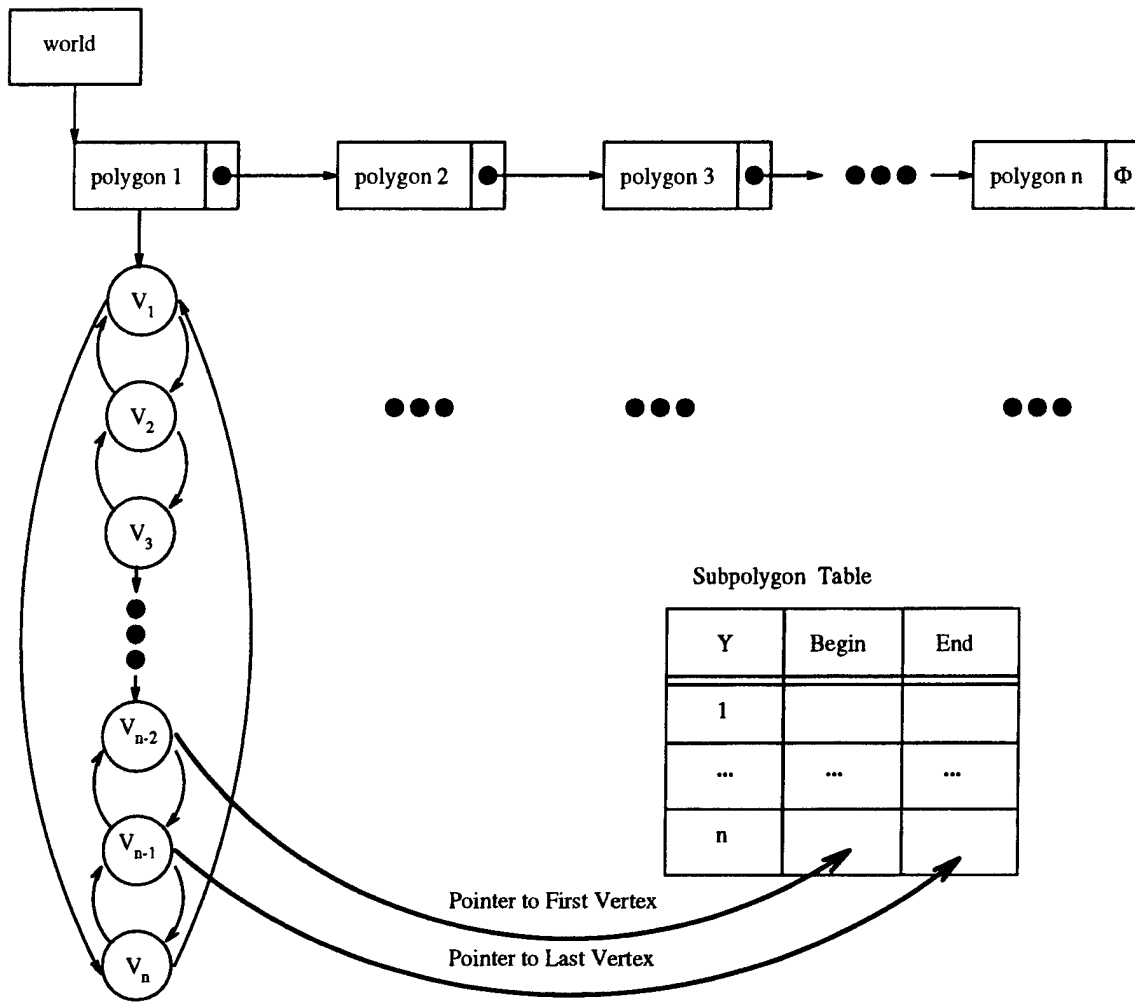
Figure 130. Representation of world data structure
