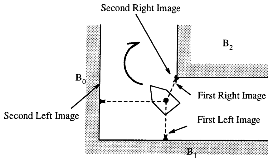
Figure 107. Right turn is required (I)
