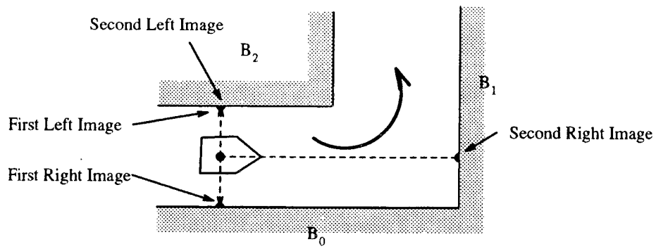
Figure 105. Left turn is required (I)
