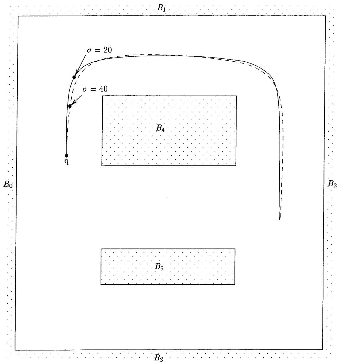
Figure 117: Motion planning and execution result (III)
