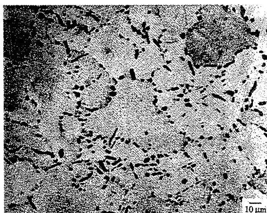
Figure 5. A356 No. 4-1 optical micrograph showing grain size at 500x.
