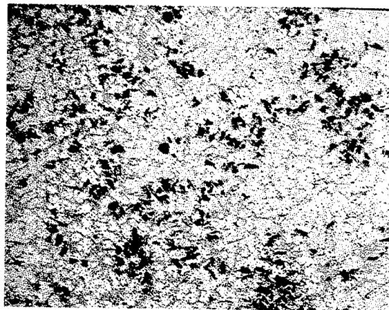
Figure 3. A359 No. 3 optical micrograph showing about 13 vol. percentage SiC reinforcement at 200x.
