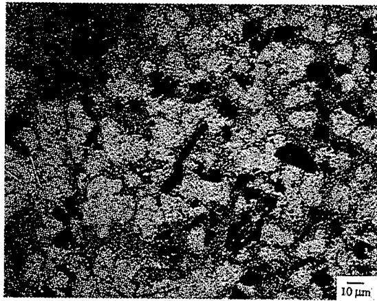
Figure 2. A359 No. 3 optical micrograph showing about 15 vol. percentage SiC reinforcement at 500x.
