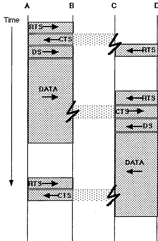
Figure 19. A Hidden-cell Network Communication Scenario
