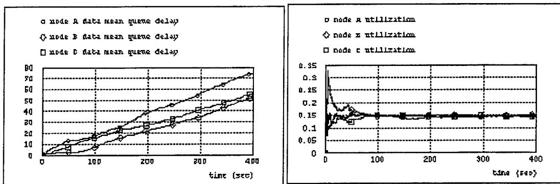
Figure 14. Hidden-Exposed Node Mean Delay and Utilization Graphs for 52% of Common Channel Load
