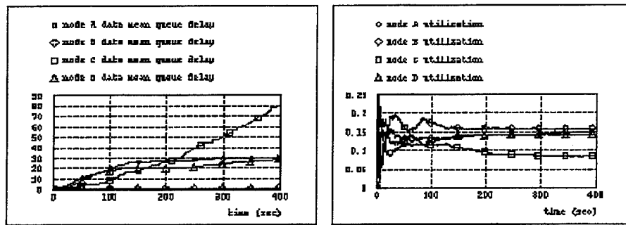
Figure 18. All-in-one Case Mean Delay and Utilization Graphs for 40% of Cell Load
