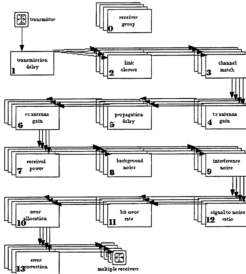
Figure 8. Radio Channel Transceiver Pipeline
