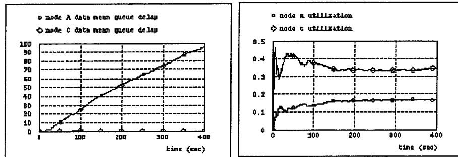
Figure 17. Hidden-Exposed Cell Mean Delay and Utilization Graph for 40% of Cell Load
