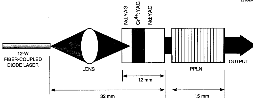
Figure 1-1. Experimental setup for optical parametric amplification of output of high-power passively Q -switched microchip laser using periodically poled lithium niobate (PPLN).
