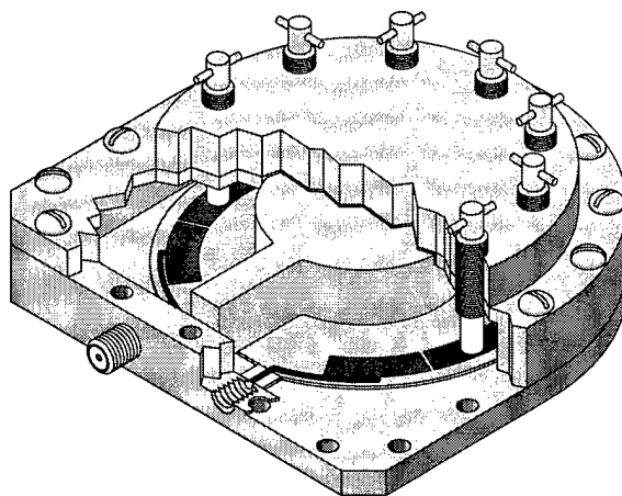
Figure 6-2. Package and tuning mechanism for a 9-pole filter. The package is made of titanium whose expansion coefficient closely matches that of \text{LaAlO}_3 .
