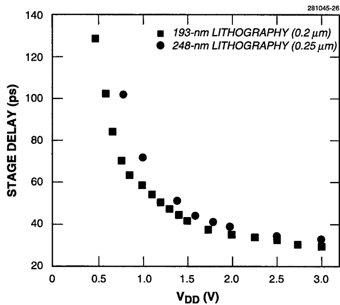
Figure 7-2. Ring oscillator stage delay vs power supply voltage.
