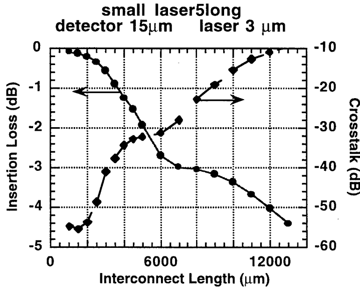
Figure F.3.1: Simulated insertion loss and crosstalk of the experimental setup as a function of longitudinal placement.
