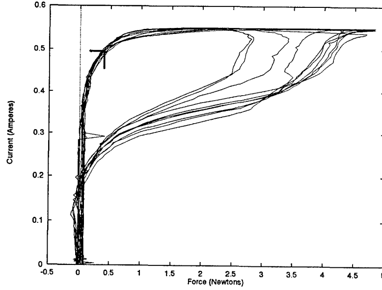
Figure 19. Cyclical Current versus Force Plot for Tactile Stimulator
