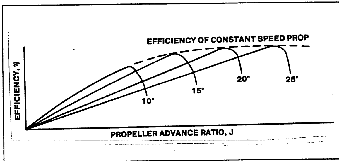
FIGURE 7.102. PROPELLER EFFICIENCY AND VARIABLE PITCH PROPELLERS
