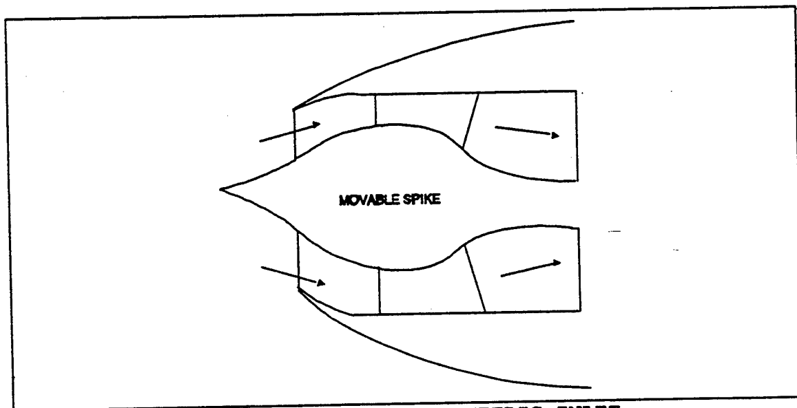
FIGURE 7.38. AXISYMMETRIC INLET
