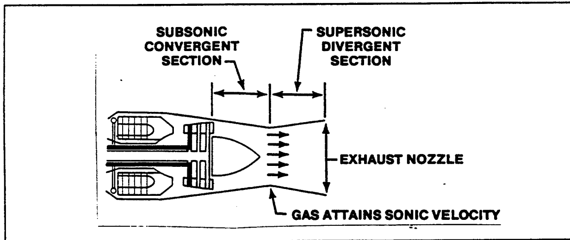
FIGURE 7.83. CONVERGENT-DIVERGENT EXHAUST DUCT (NOZZLE)
