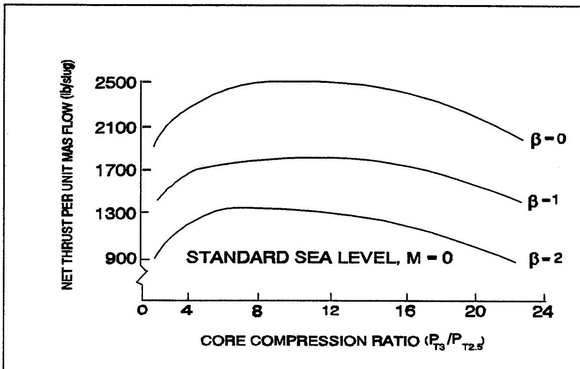
FIGURE 7.29. EFFECT OF CORE COMPRESSION RATIO ON NET THRUST FOR THE TURBOFAN ( TIT=2400^{\circ}R AND CR_f=2 )
