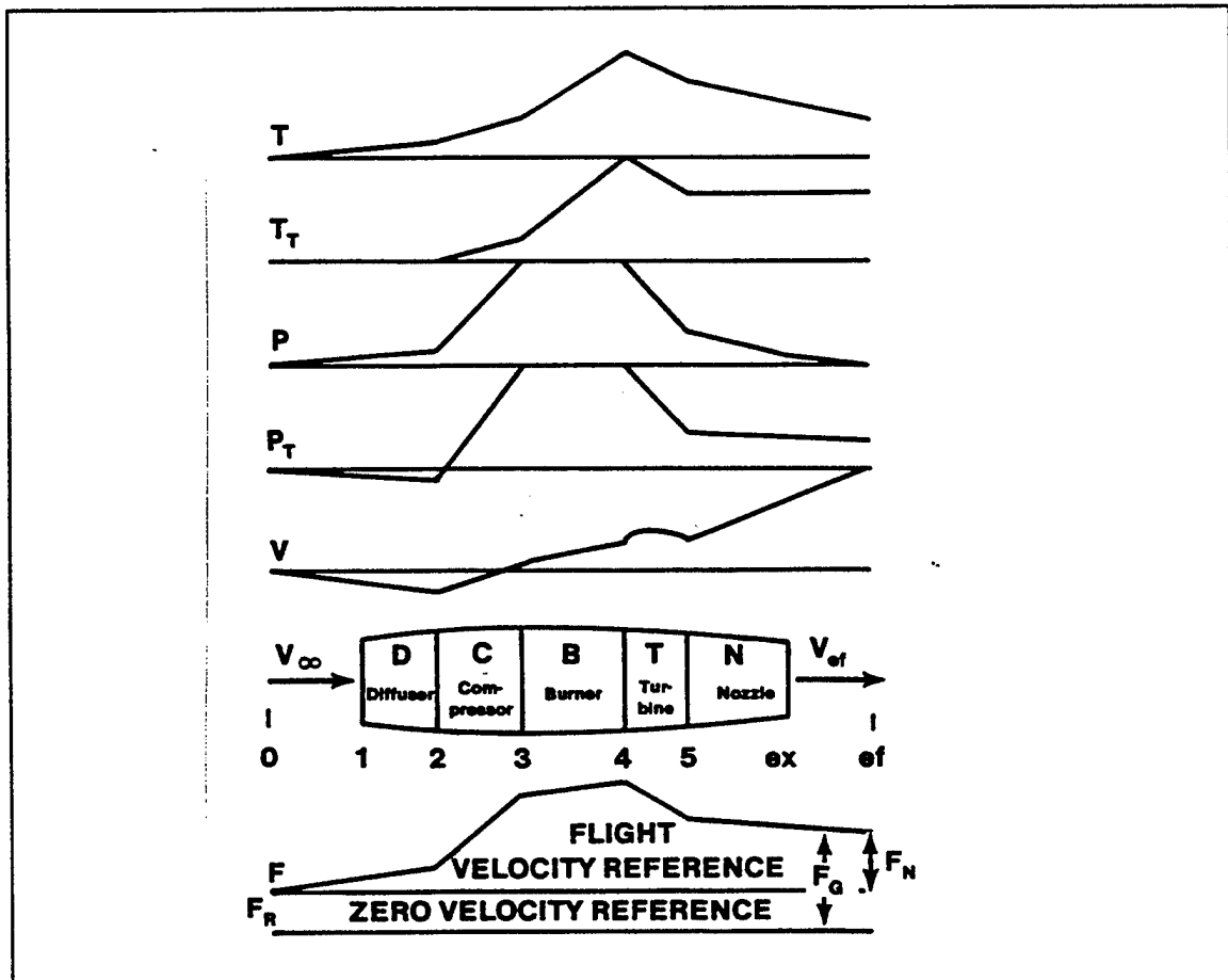
FIGURE 7.87. VARIATION OF GAS PROPERTIES THROUGH A TURBOJET ENGINE DURING FLIGHT
