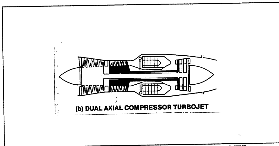
FIGURE 7.5B. DUAL AXIAL COMPRESSOR TURBOJET
