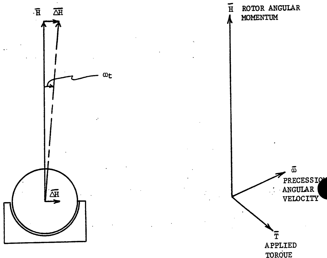
FIGURE 9.21 GYRO VECTORS
