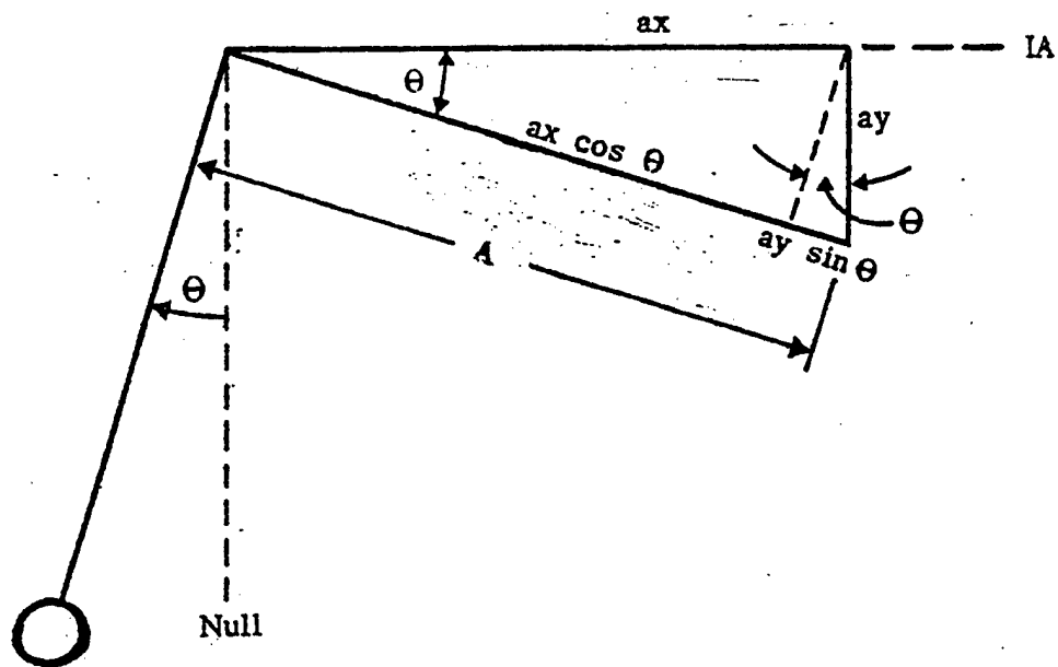
FIGURE 9.17. CROSS COUPLING
