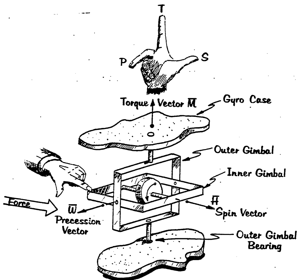
FIGURE 9.19. PRECESSION OF A TWO DEGREE OF FREEDOM GIMBALED GYRO
