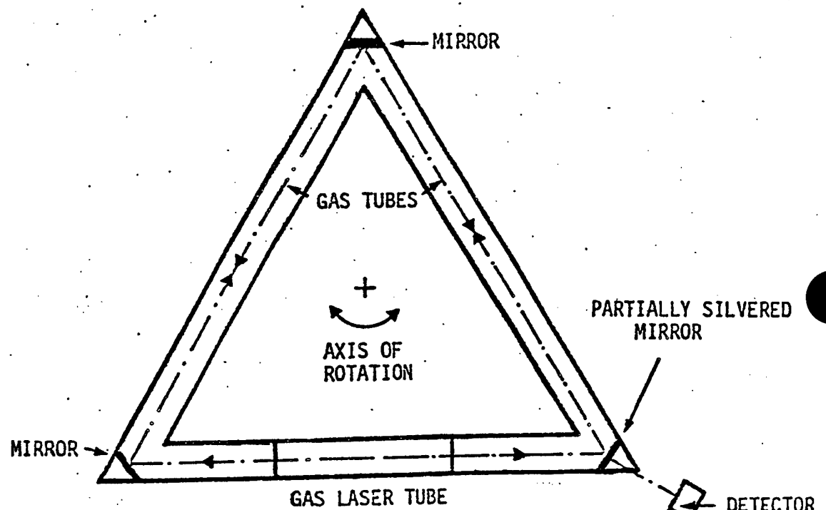
FIGURE 9.31. LASER GYRO
