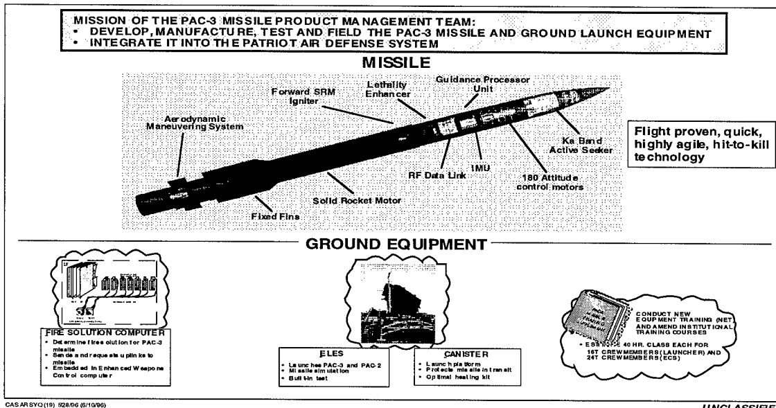
Figure 2. PAC-3 Missile Products
