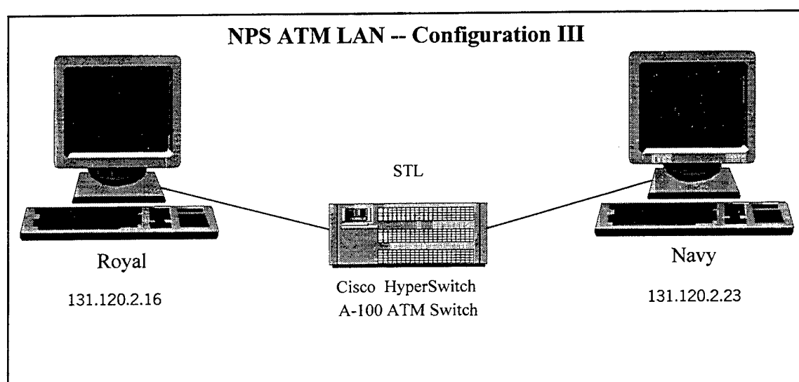
Figure 76. Single-Switched ATM LAN.
