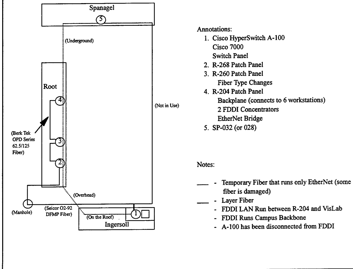
Figure 3. NPS Campus Backbone Topology, after [Romo, 1995].
