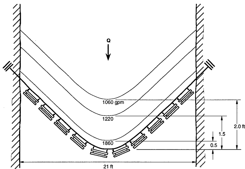
Figure 10. Water surface velocity distribution just upstream of a boom.
