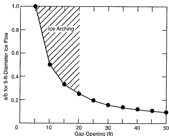
Figure 2. Gap opening vs. a/b value for a floe 5.0 ft (1.5 m) in diameter. The opening must be 20.0 ft (6.1 m) or less for an arch to form.
