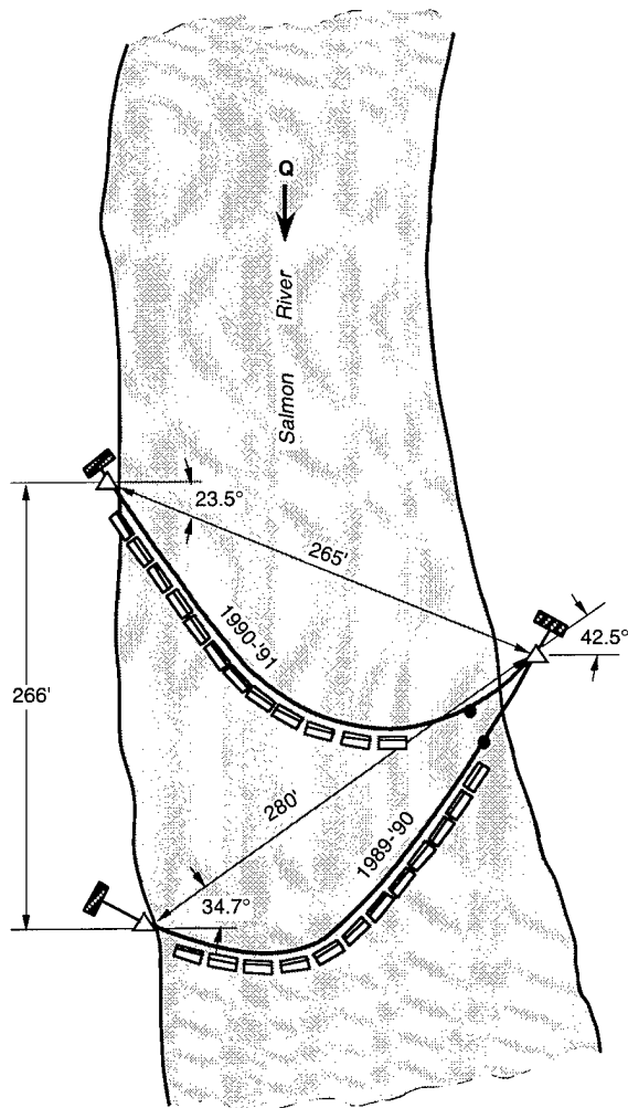
Figure 7. Salmon River ice boom geometry.
