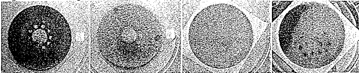
FIGURE 2a. Hafnium Carbide Wafer M15 Front FIGURE 3a. Hafnium Carbide Wafer M13 Front FIGURE 4a. Hafnium Carbide Wafer M11 Front FIGURE 5a. Hafnium Carbide Wafer M1 Front
