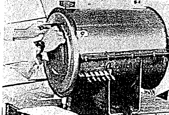
FIGURE 7. Jacketed RVCC Experimental Hardware Showing Wafer Insertion
