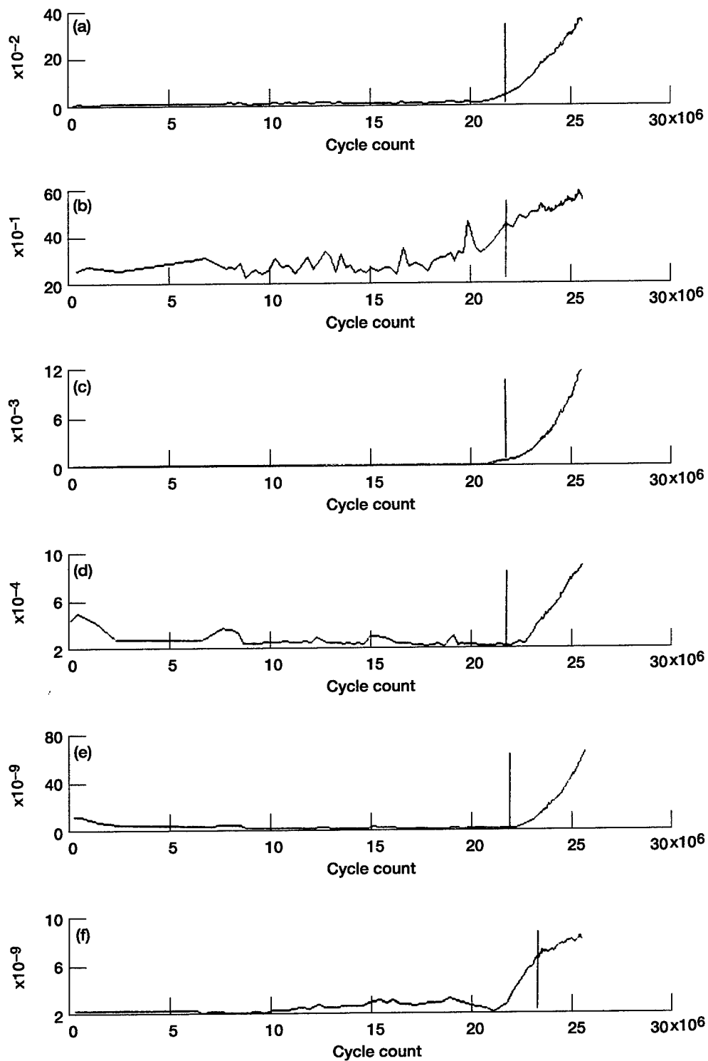
Figure 13.—Features plots for test run B. (a) Peak residual pinion stresswave. (b) Kurtosis pinion stresswave. (c) Total energy pinion stresswave. (d) Peak residual gear baseband stresswave. (e) Total energy gear baseband envelope. (f) Kurtosis gear stresswave.
