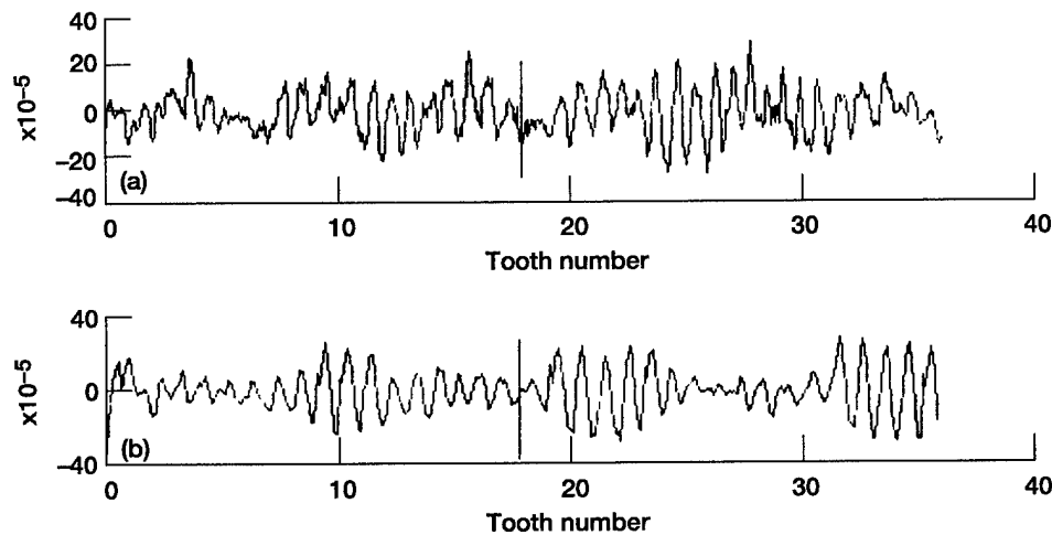
Figure 8.—Time synchronous average plots of gear for test run A. (a) Gear raw baseband plot. (b) Gear baseband envelope.
