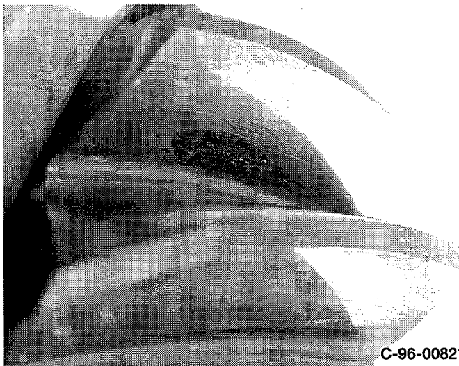
Figure 15.—Gear and pinion fatigue spall for test run C.
