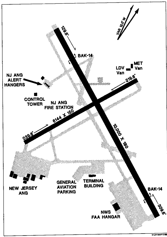
FIGURE 3-2. LDV INSTALLATION AT FAA TECHNICAL CENTER
