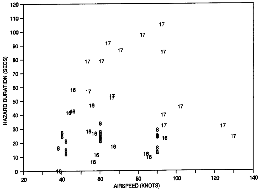
FIGURE 4-13. S-76A MODELED VORTEX HAZARD DURATION VS. AIRSPEED (KNOTS)
