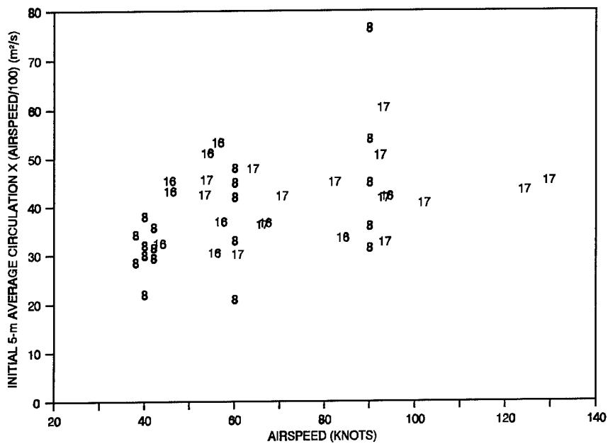
FIGURE 4-5. S-76A 5-M INITIAL AVERAGE CIRCULATION X (V/100) VS. AIRSPEED (KNOTS)
