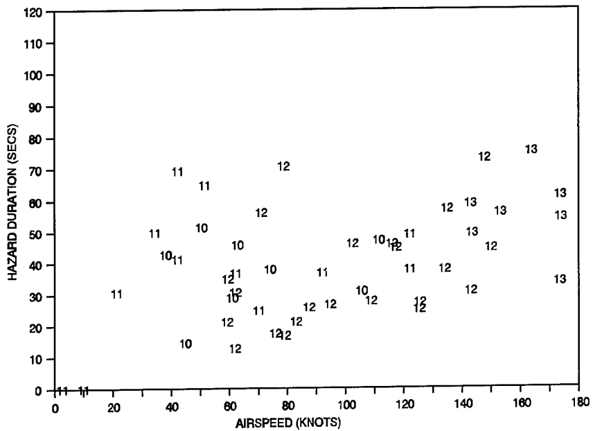
FIGURE 4-14. UH-60A MODELED VORTEX HAZARD DURATION VS. AIRSPEED (KNOTS)
