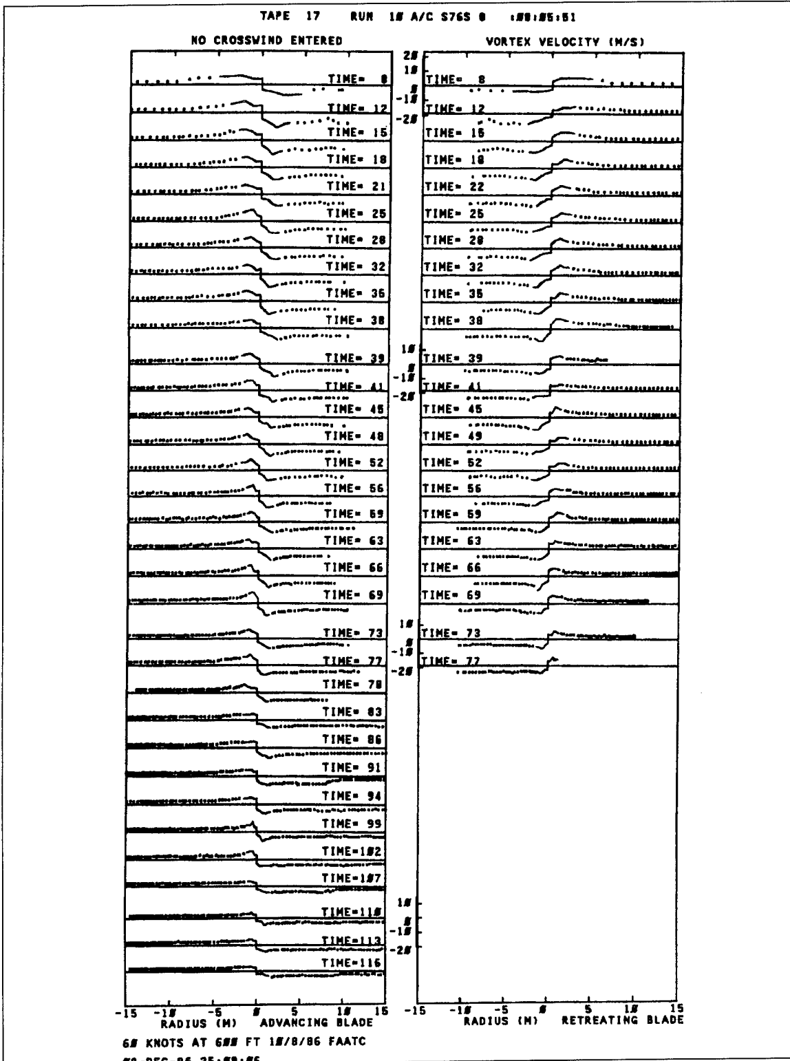
FIGURE 3-8. S-76A VELOCITY PROFILE TIME HISTORY
