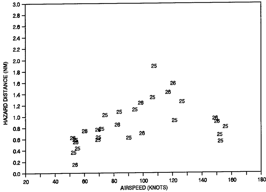
FIGURE 4-18. UH-60A PREDICTED VORTEX HAZARD DISTANCE (NM) VS. AIRSPEED (KNOTS)
