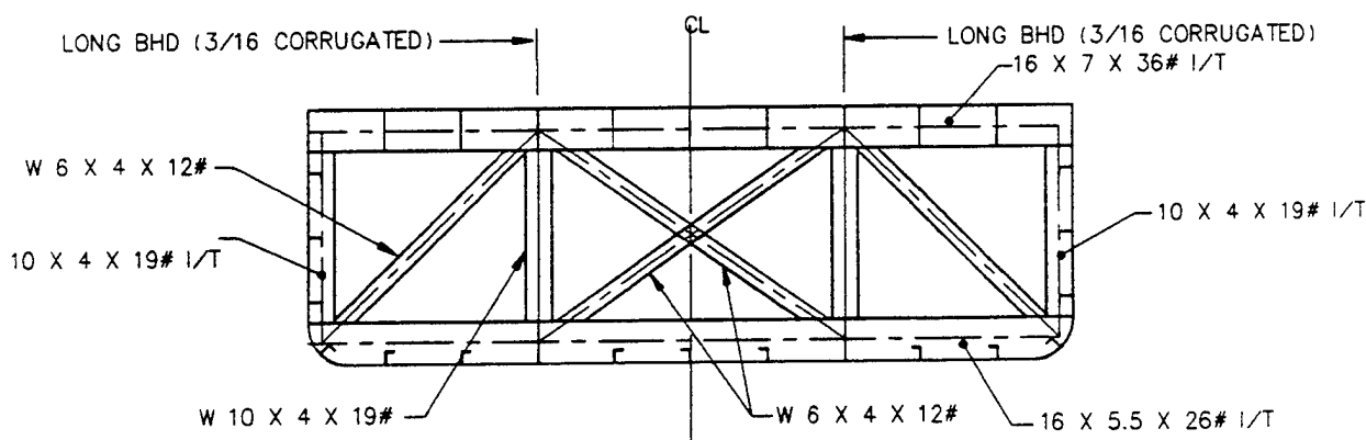
SECTION E-E TYPICAL TRUSS
