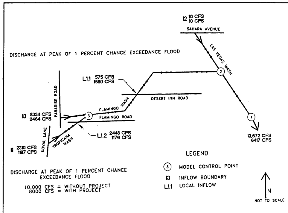
Figure 31. Hydrology input schematic, for HEC-6W numerical model
