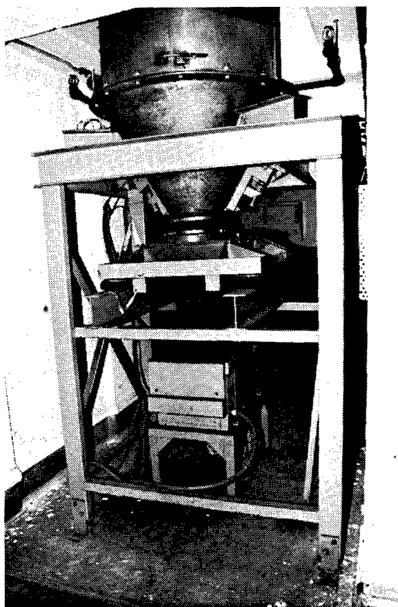
Figure 128. Building 6704-4: Hopper and scale where paste, dispensed by the hopper, was weighed in 50-pound increments and bagged.
