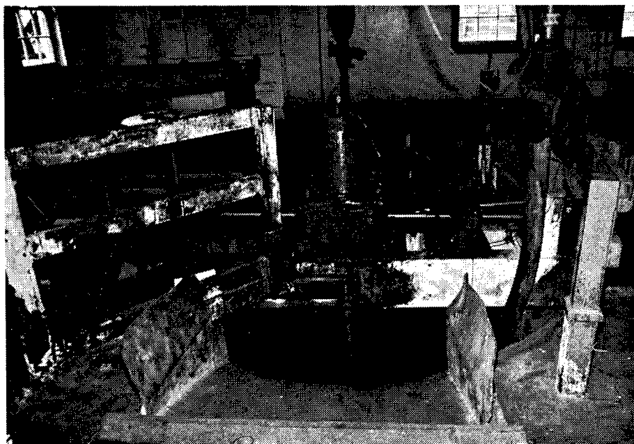
Figure 123. Building 6702-4: Mixer for the paste or slurry compound (nitrocellulose, nitroglycerin, and water).
