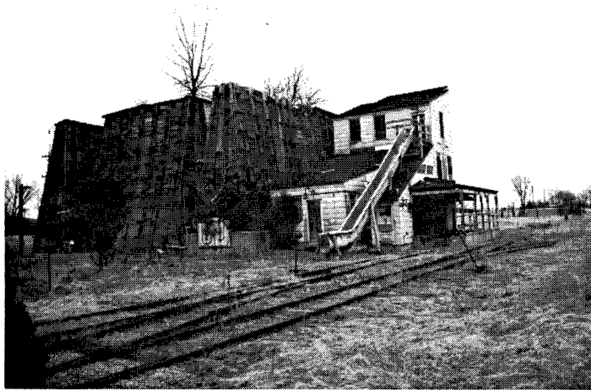
Figure 140. Building 6731-4: Barricaded Paste Breaker and Blender House. The main building area is separated by a double riveted barricade from the tram loading dock and the platform/elevator structure.
