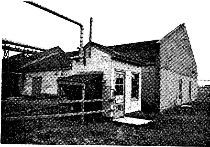
Figure 85. Building 2513-4: Horizontal Press House that had end-walls constructed of reinforced concrete extended above the roof.
