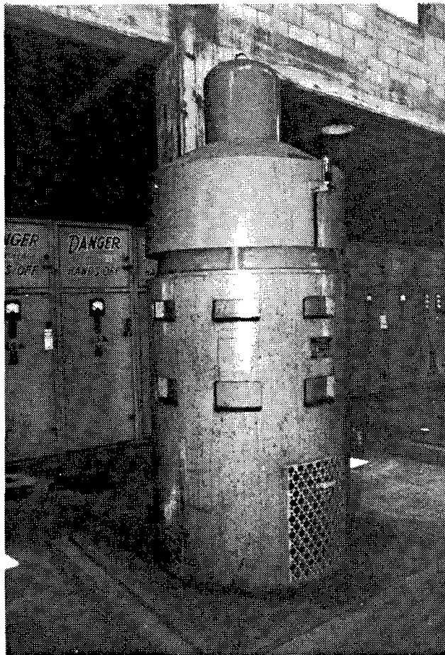
Figure 351. Building 408: Another vertical turbine pump with a 500 HP engine and 100,000 gallons per minute capacity, manufactured in 1942 by Ponomo.
