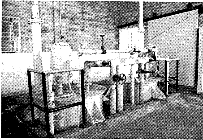
Figure 198. Building 9501-3: Interior view of the second floor showing a colloid and salt tank manufactured in 1954.
