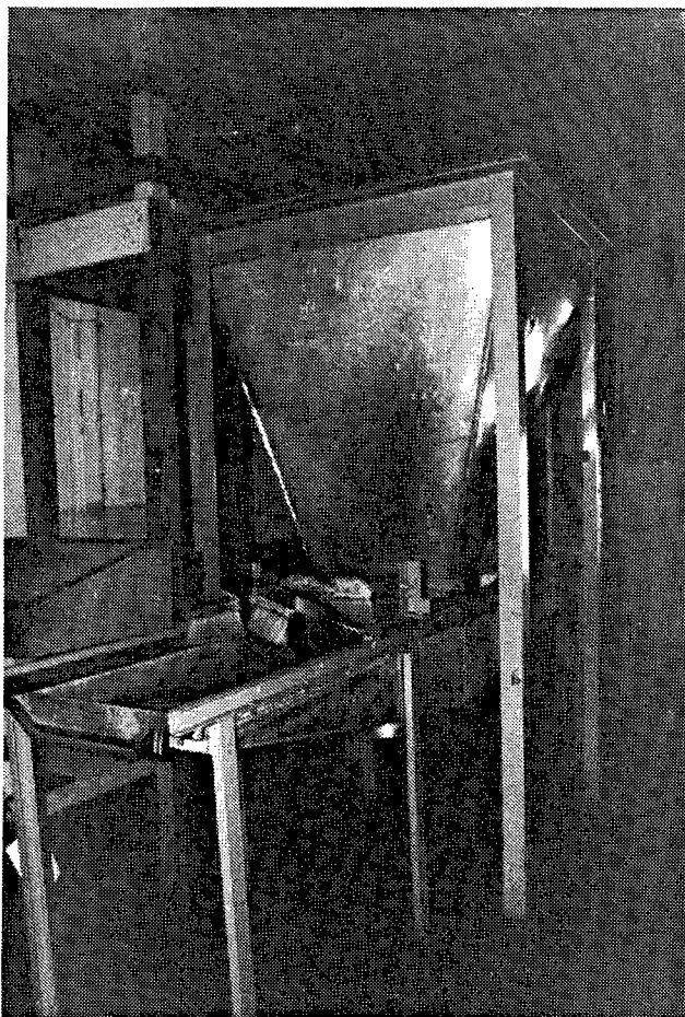
Figure 217. Building 9513-2: Tray loading unit that includes hopper and table, manufactured in 1955.
