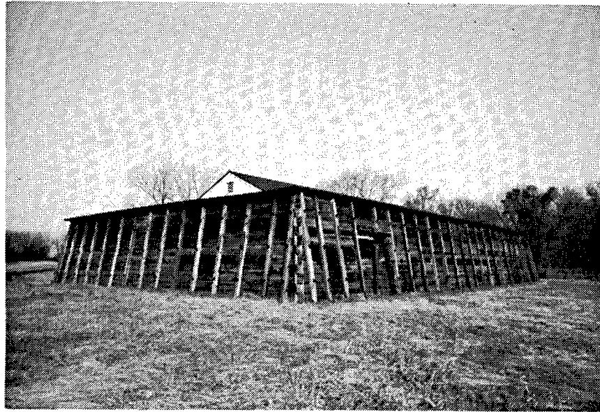
Figure 319. Building 1906-10: Barricaded Magazine. The barricades were designed to direct an explosion upward rather than outward. An outward explosion could trigger additional explosions in neighboring magazines.
