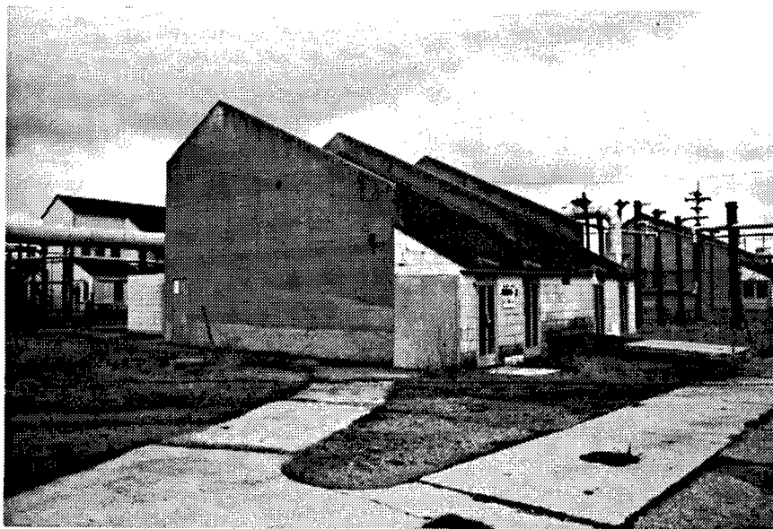
Figure 79. Building 4510-2: Block Press House that has reinforced concrete walls dividing the building into three areas.
