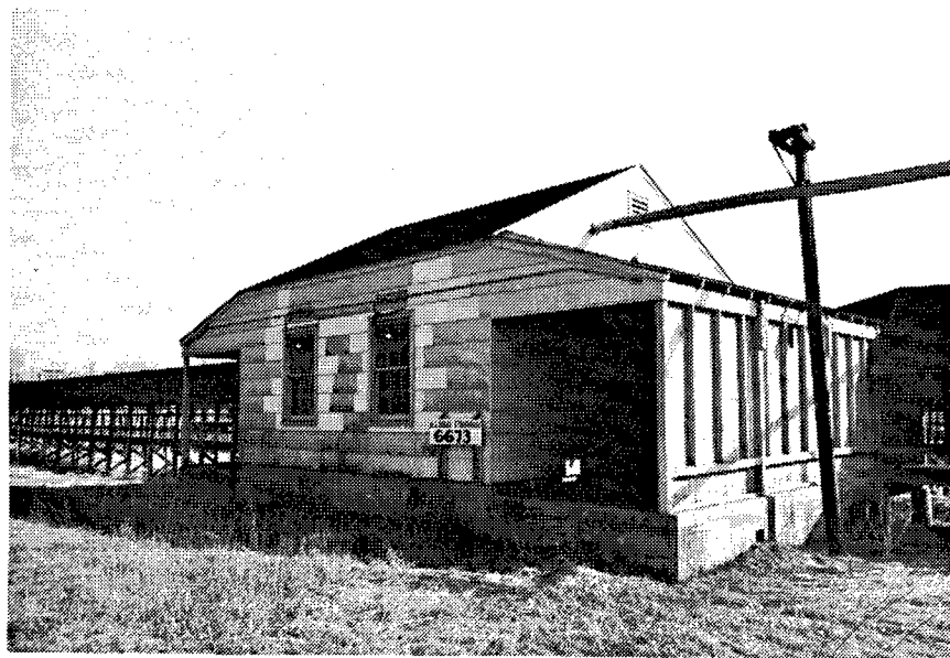
Figure 291. Building 6673: Nitroglycerin Buggy Storehouse.
