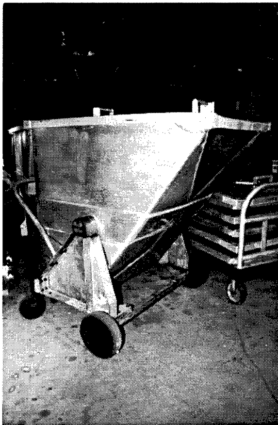
Figure 118. Building 6701: Buggy with crank to aide in tilting the buggy's barrel on the first level.
