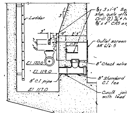
SECTION E-E SCALE: 1/2 IN. = 1 FT.
