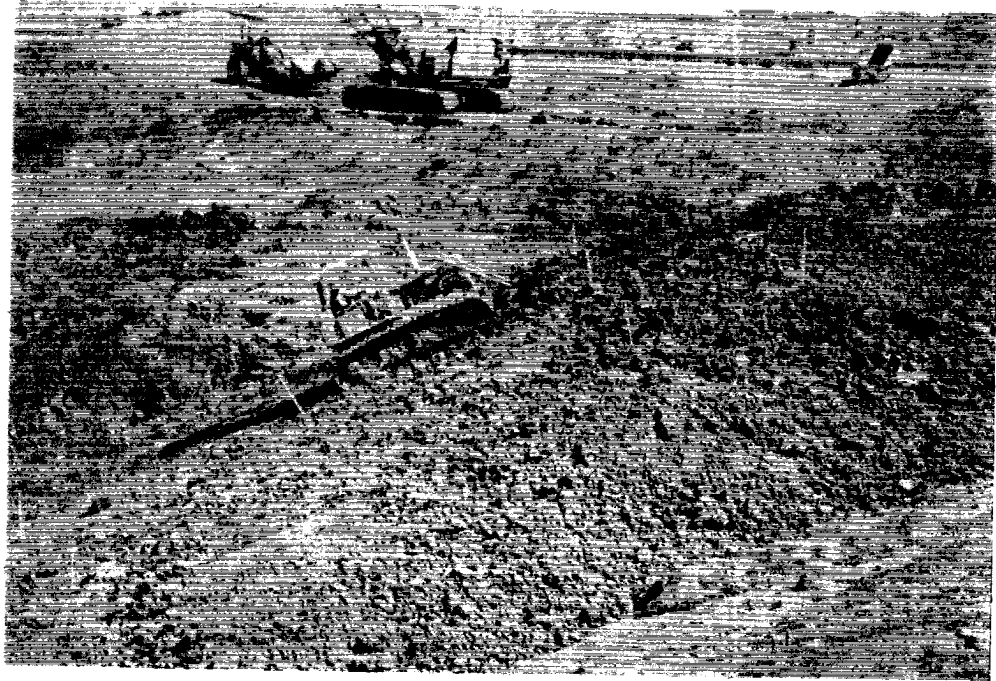
17. COMPACTING IMPERVIOUS BACKFILL NORMAL TO 1 ON 2 SLOPE
