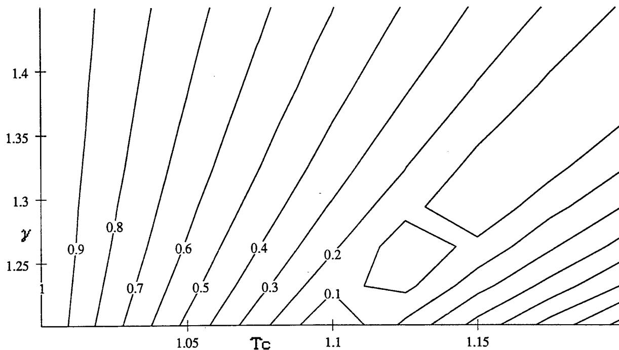
Figure 5-12 (K 2 ) Direct Influence of \tau on Supply Tank Mass Flow Uncertainty
