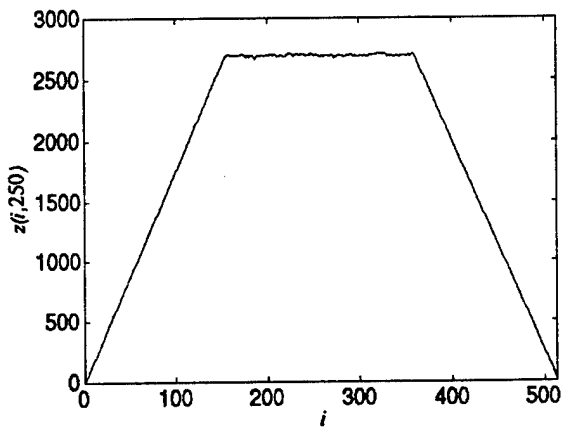
Figure 3. Cross Section of Sand Pile Structure for \sigma_c = 20 and N = 7 \times 10^8 .
