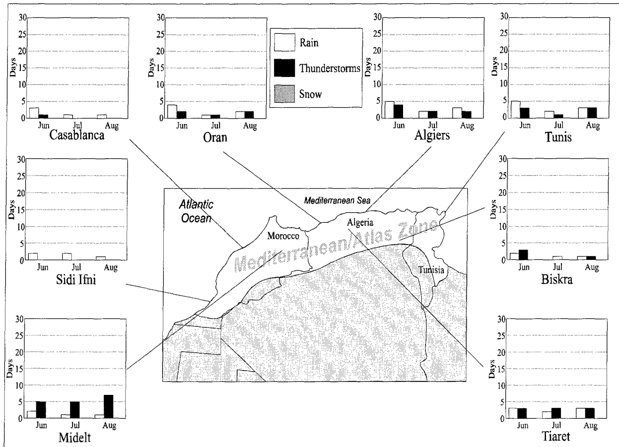
Figure 3-26. Summer Mean Precipitation and Thunderstorm Days. The graphs show the average summertime occurrence of rain and thunderstorm days for selected cities in the Mediterranean/Atlas zone.
