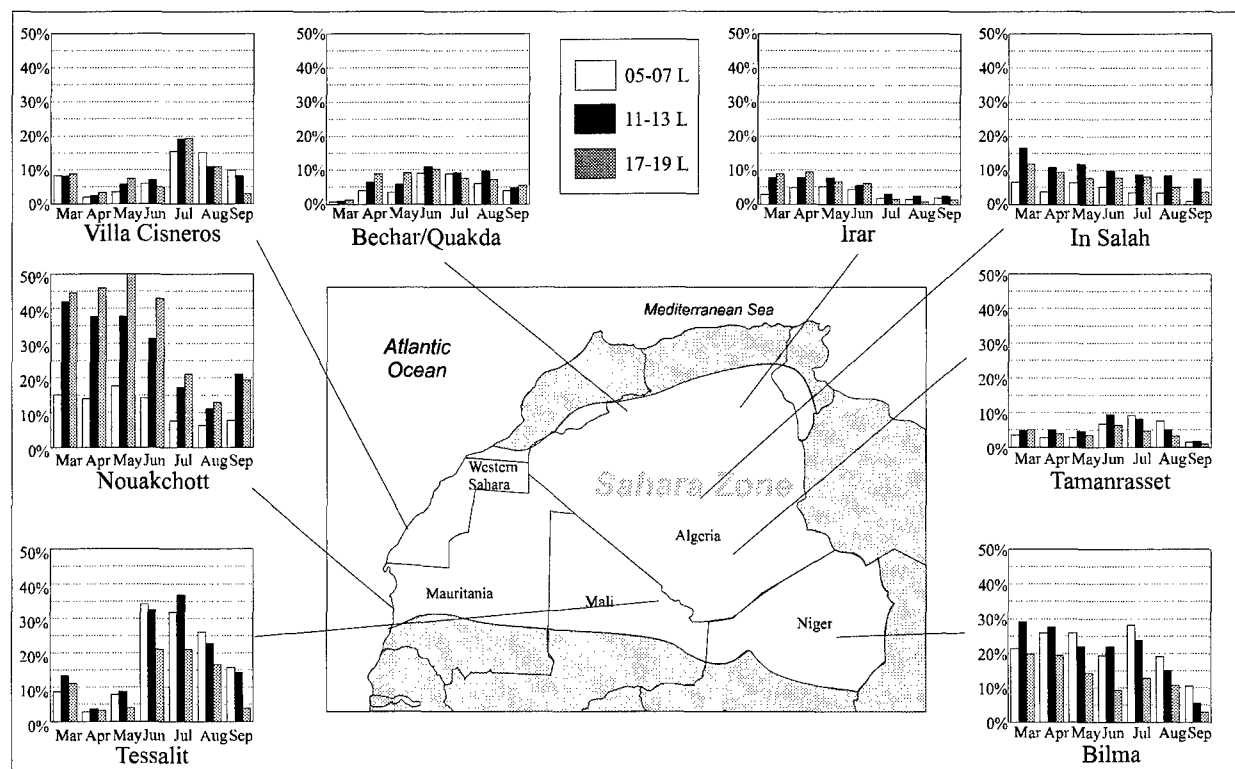
Figure 4-4. Summer Percent Frequencies of Visibilities Below 4,800 Meters. The graphs show a monthly breakdown on the percentage of visibilities below 4,800 meters based on location and diurnal influences.
