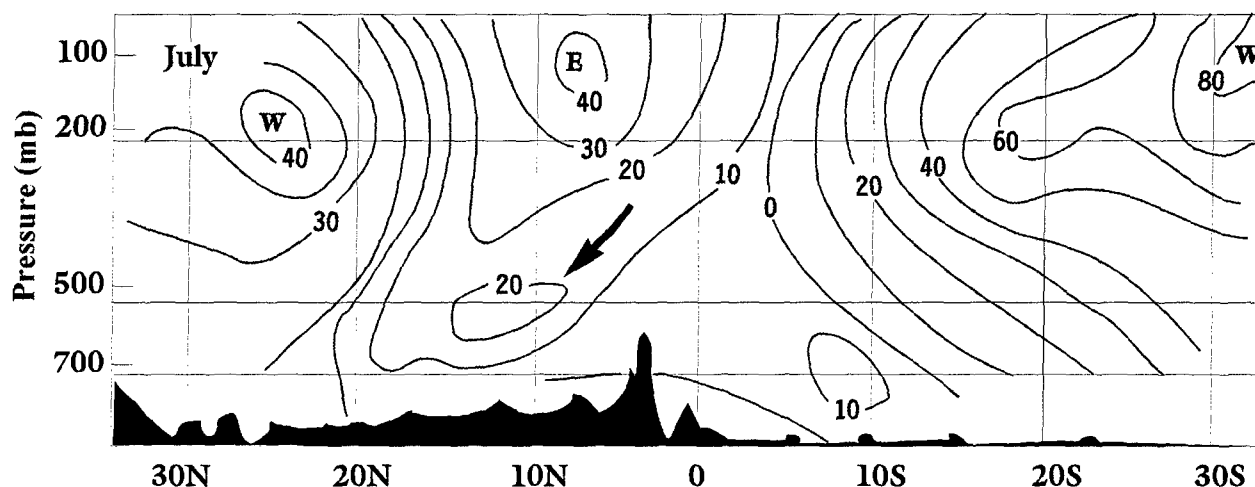
Figure 2-9. North-South Cross Section of Zonal Winds near 10^{\circ} E for July. Solid lines are isotachs in knots; the arrow shows the location of the MTEJ. Terrain features are shown at bottom of figure.
