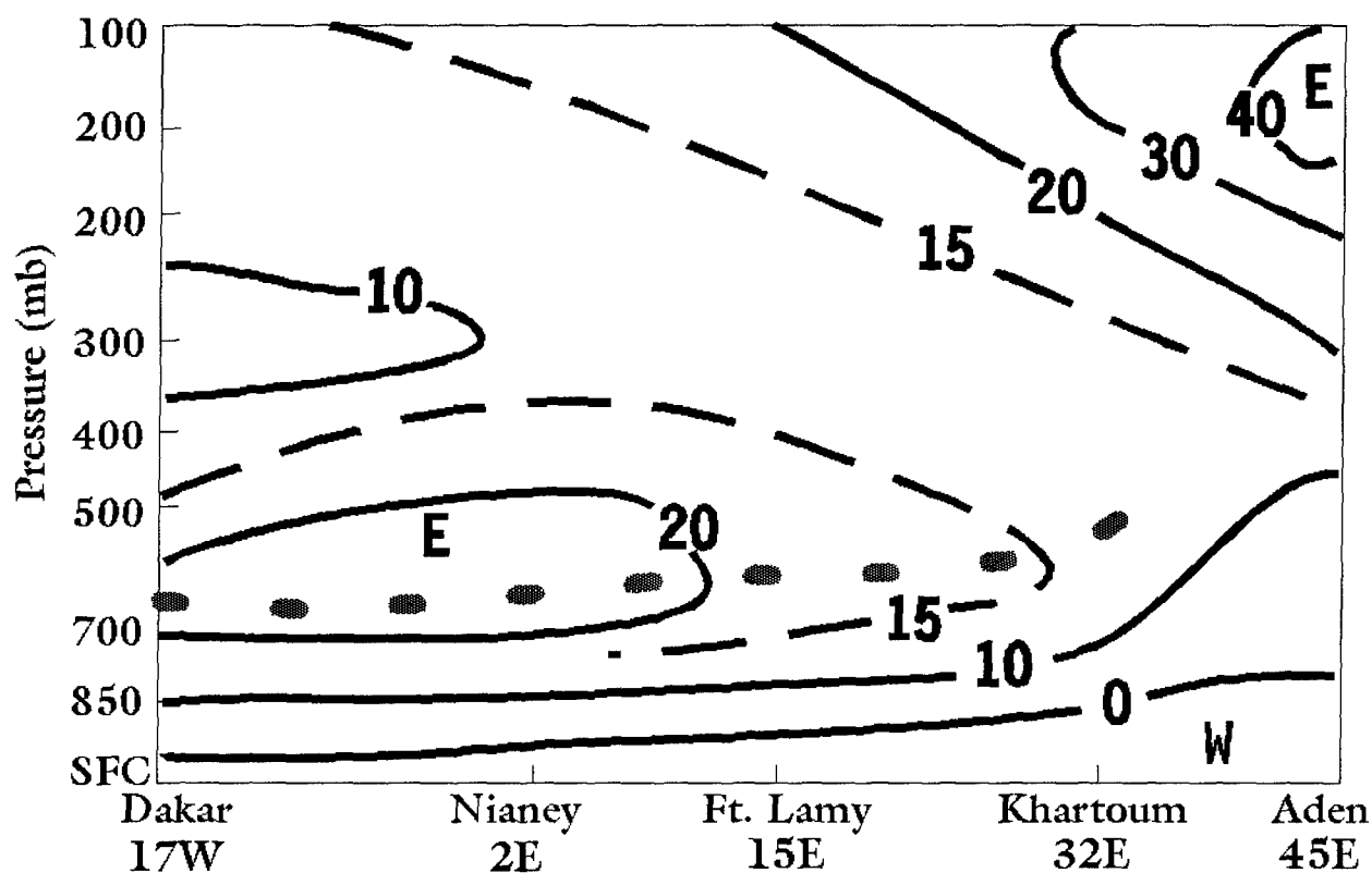
Figure 2-10. West-East Cross Section Showing the MTEJ at 13^{\circ} N in August (Burpee, 1972). Solid lines are isotachs in 10 knot increments; dashed lines are isotachs in 5 knot increments. The dotted line shows the jet axis.
