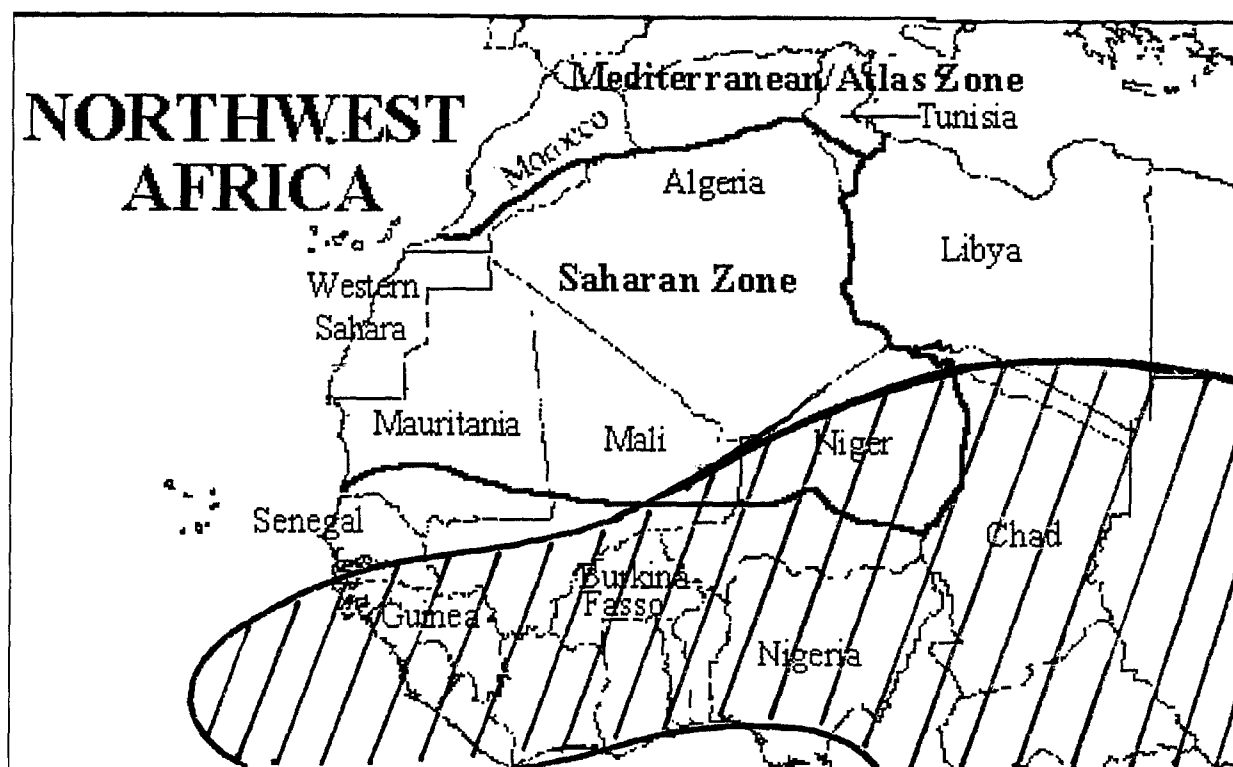
Figure 2-4. Monsoon Climate (hatched area) Across Africa (Ramage, 1971). Figure shows the portion of Northwest Africa affected by the monsoon climate.
