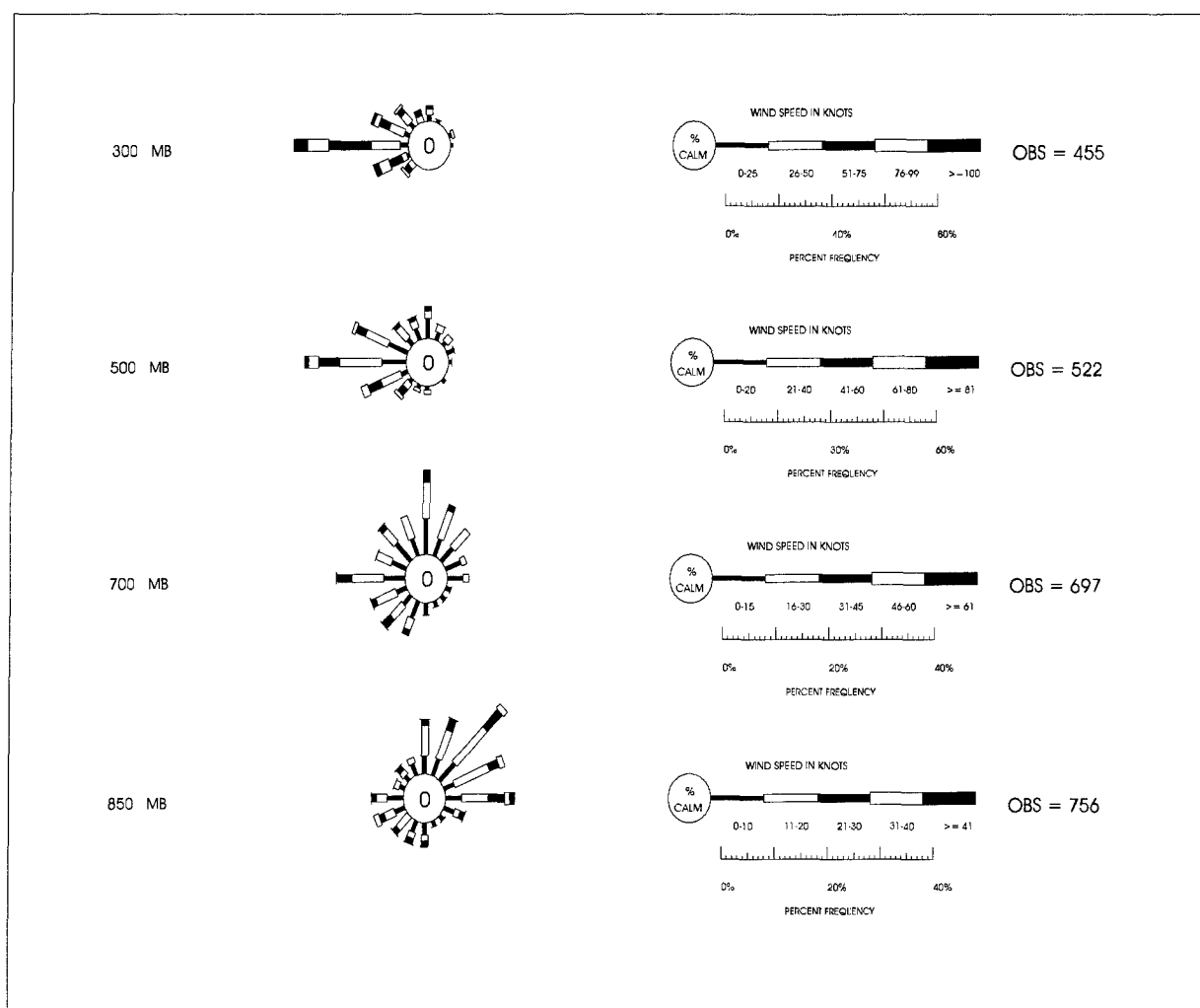
Figure 4-15. January Upper-Air Wind Roses. The wind roses depict wind speed and direction for standard pressure surfaces between 850 and 300 mb at In Salah, Algeria.
