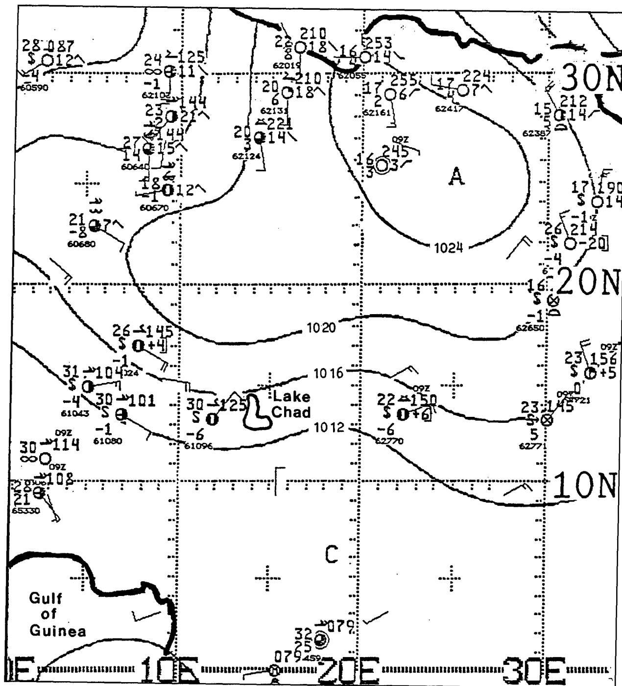
Figure 2-22. Surface Chart of Harmattan-Produced Duststorm over North Africa March 6, 1991. Wind barbs without station data are satellite-derived. Note the dusty conditions associated with the southern quadrant of the anticyclone.
