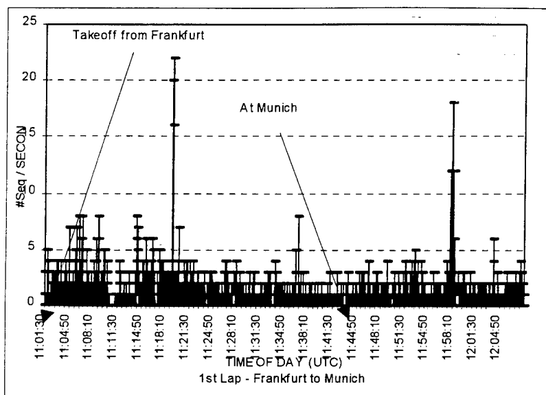
FIGURE 8. MODE 4 INTERROGATIONS
