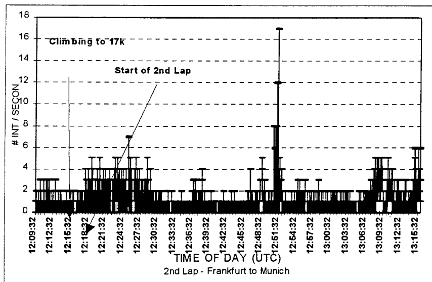
FIGURE 9. MODE 4 INTERROGATIONS
