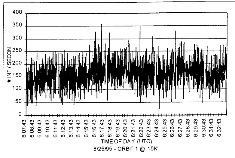
FIGURE 29. UNSUPPRESSED MODE A INTERROGATIONS
