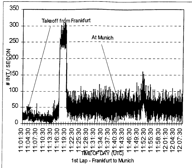
FIGURE 11. MODE C INTERROGATIONS
