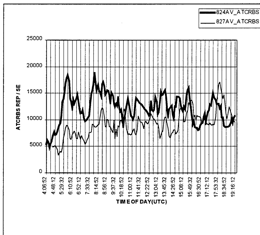
FIGURE 37. ATCRBS REPLY RATES - FRANKFURT, GERMANY
