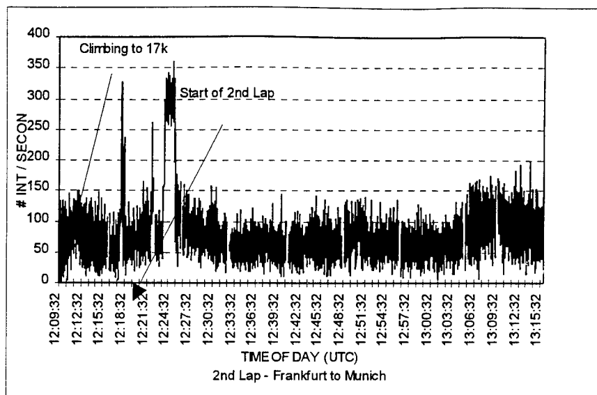
FIGURE 16. MODE C INTERROGATIONS
