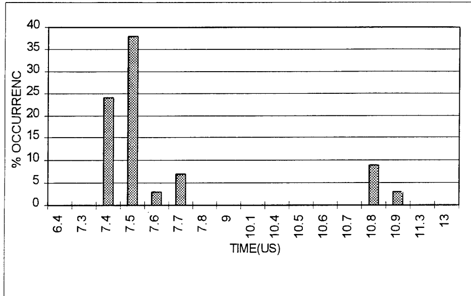
FIGURE 21. TIME DIFFERENCE OF MODE 2 AND PRECEDING INTERROGATIONS FROM RADAR #36
