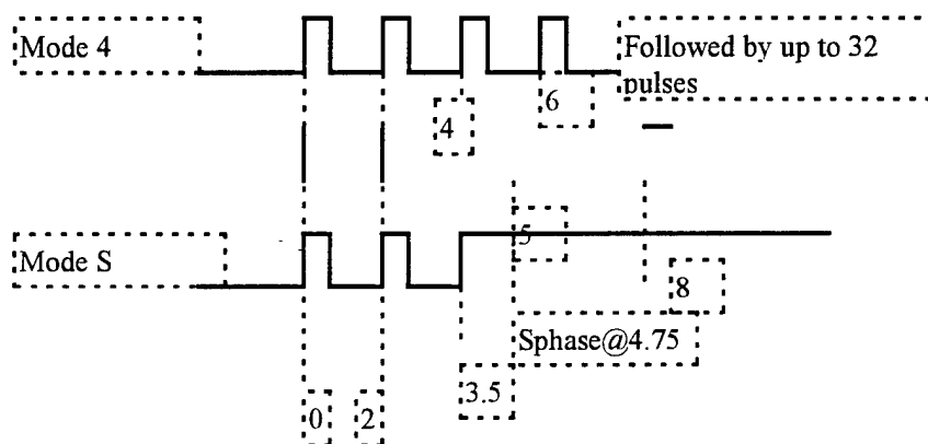
FIGURE 1. FALSE MODE 4'S FROM MODE S INTERROGATIONS
