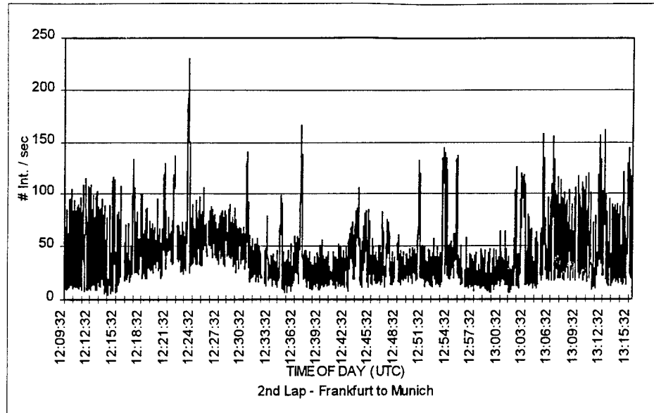
FIGURE 18. MODE 2 INTERROGATIONS
