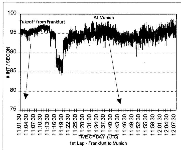
FIGURE 14. TRANSPONDER AVAILABILITY
