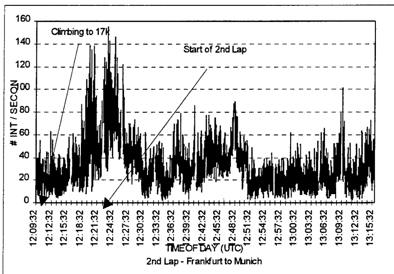
FIGURE 15. MODE S INTERROGATIONS
