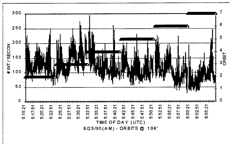
FIGURE 31. MODE S INTERROGATIONS
