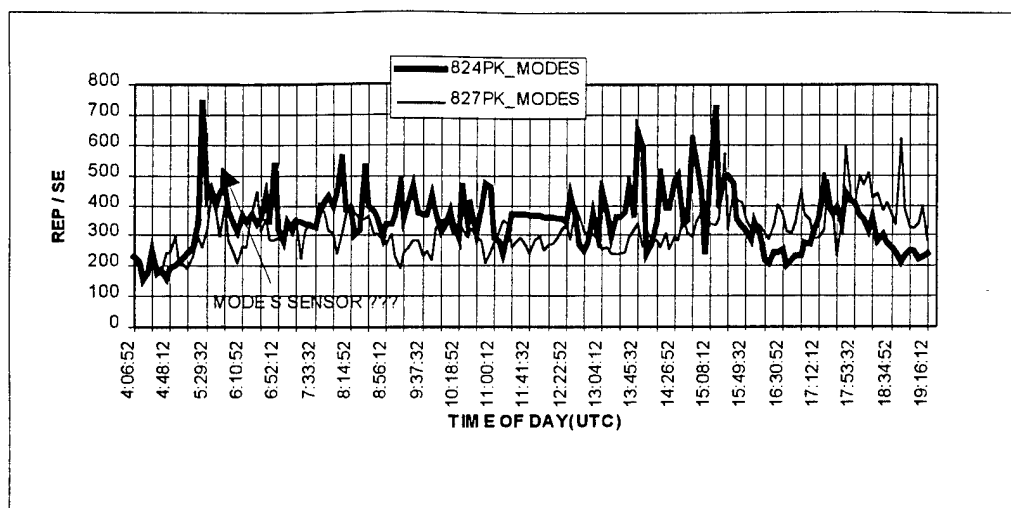
FIGURE 40. MODE S PEAK REPLY RATES - FRANKFURT, GERMANY
