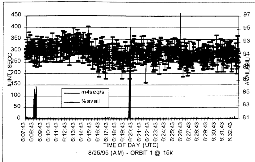
FIGURE 25. MODE 4 INTERROGATION SEQUENCES
