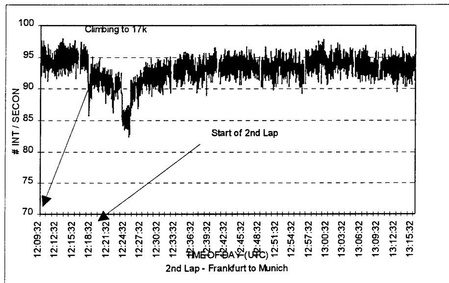
FIGURE 19. TRANSPONDER AVAILABILITY
