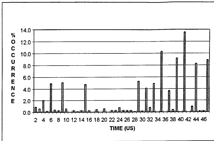
FIGURE 2. TIME DIFFERENCE - FIRST TO LAST MODE 4 INTERROGATIONS
