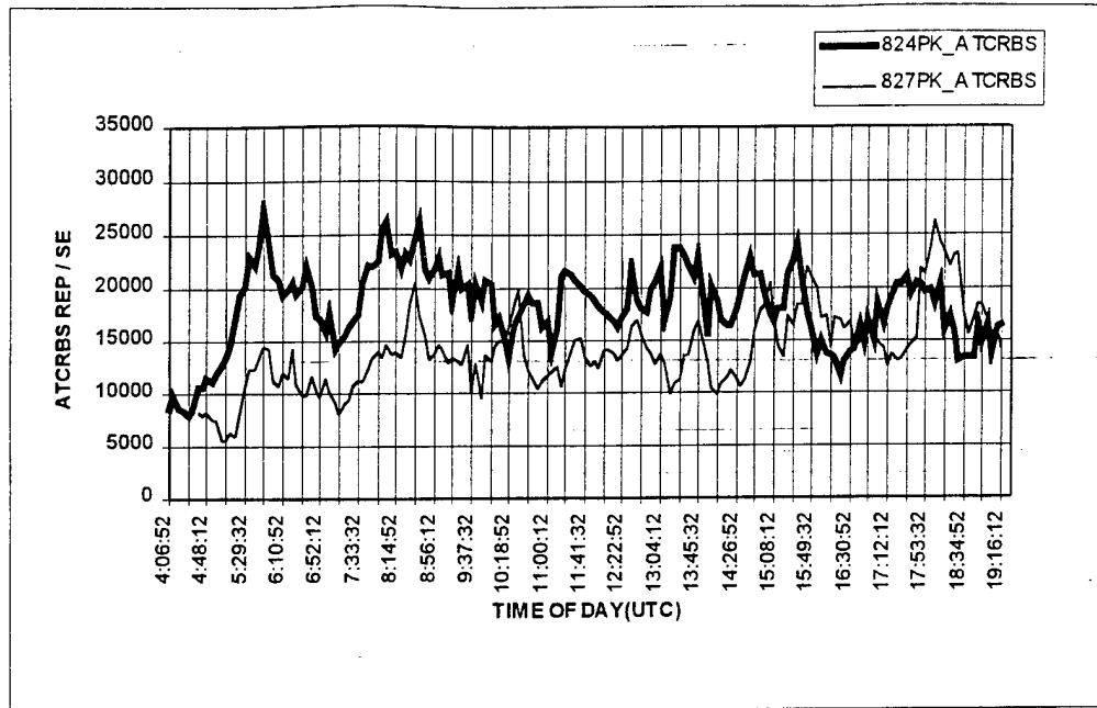
FIGURE 38. ATCRBS PEAK REPLY RATES - FRANKFURT, GERMANY
