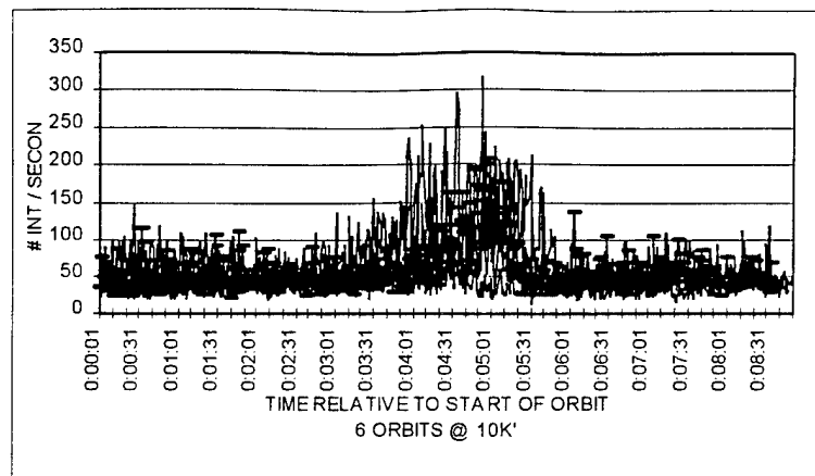
FIGURE 35. UNSUPRESSED MODE 2 INTERROGATIONS
