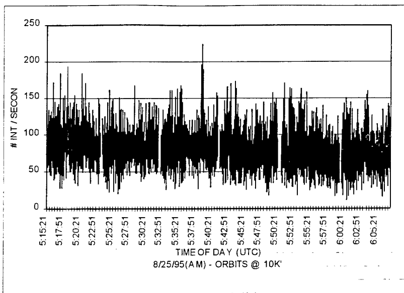
FIGURE 33. UNSUPPRESSED MODE C INTERROGATIONS
