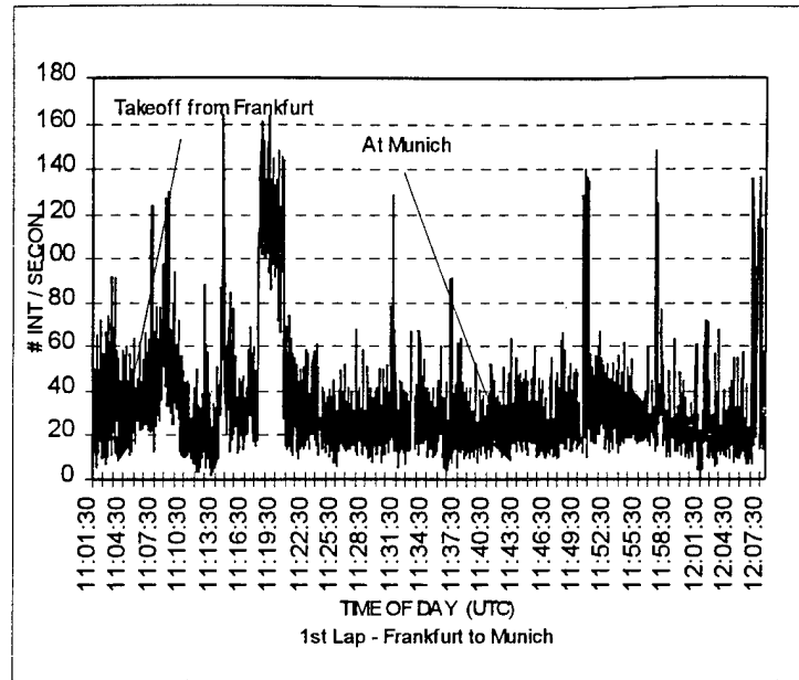
FIGURE 13. MODE 2 INTERROGATIONS
