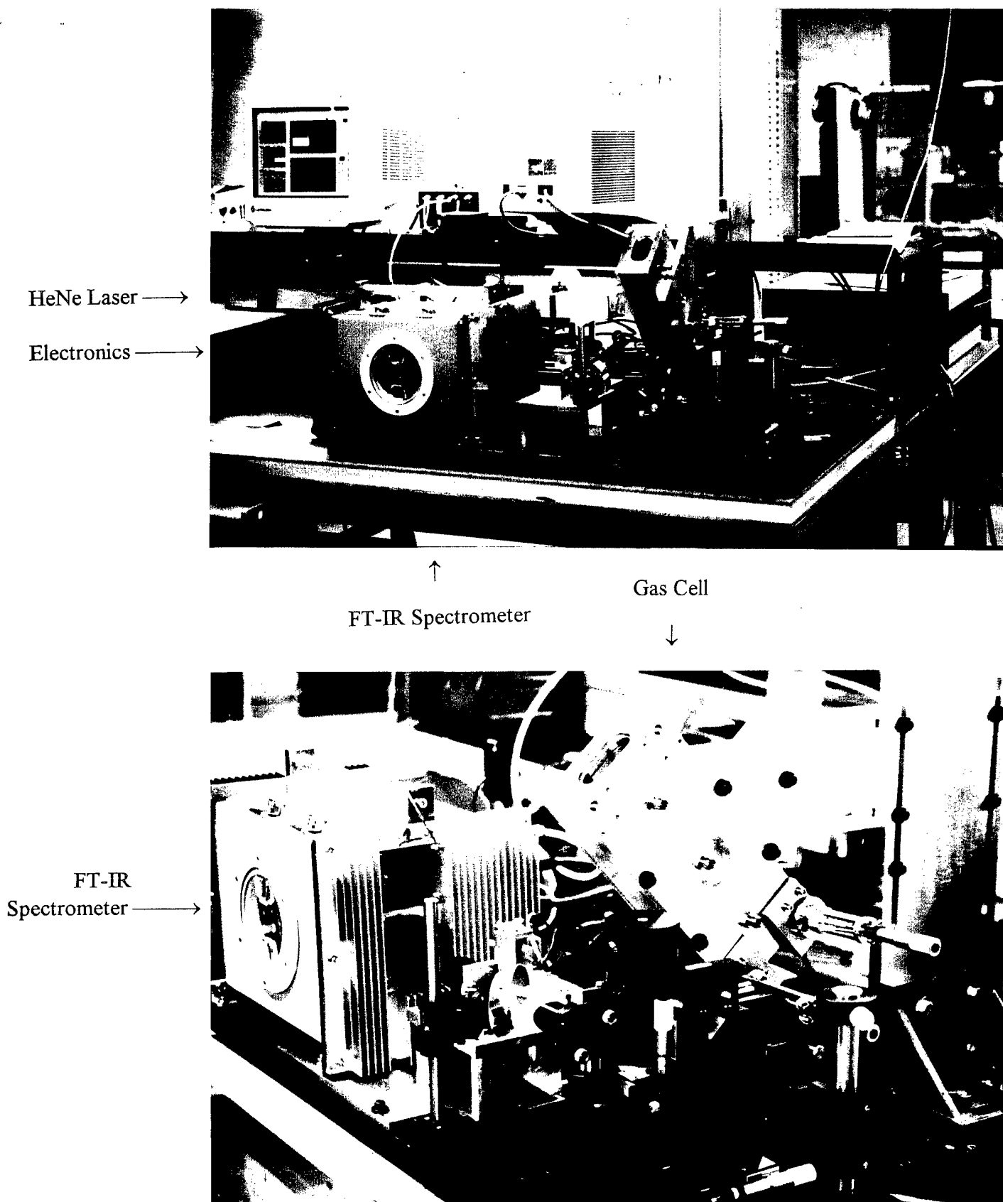
Figure 3. Photographs of Phase I Optical Assembly (less end-cap mirrors on gas cell). The Black Optical Platform with the Many Tapped Holes is 36" x 24" x 1/2" Thick. The Opening on the Gas Cell for the Objective Mirror is Seen.
