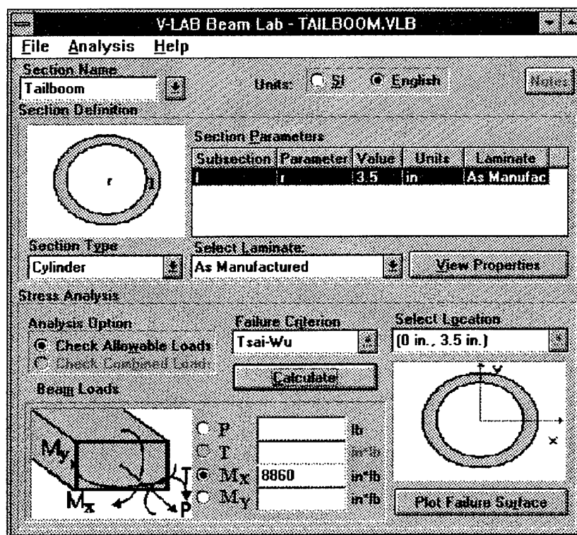
Figure 13—Beam Lab Models the Tailboom Using Cylindrical Shell with Nominal and As-Manufactured Configurations of the Laminate
