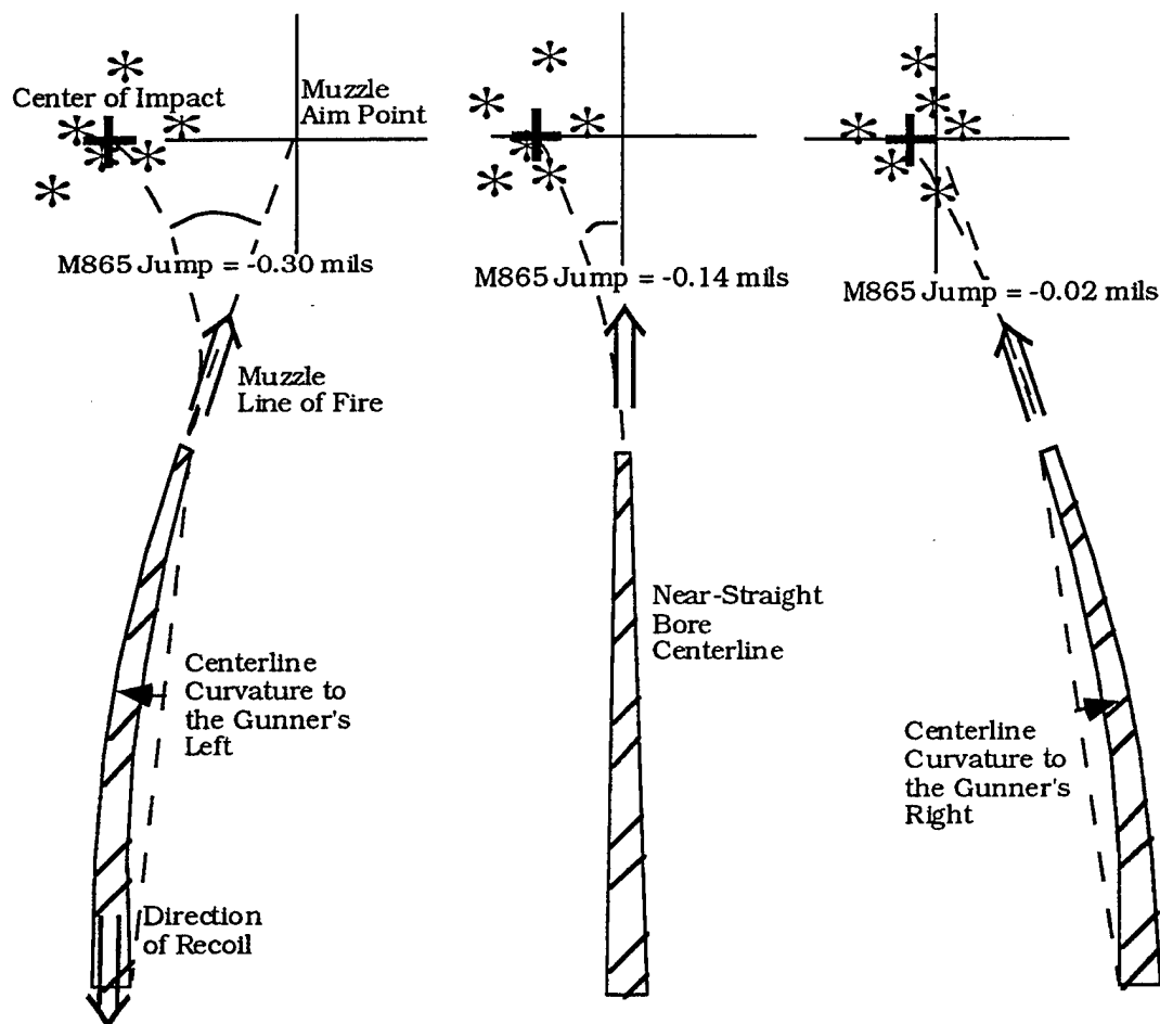
Figure 8. Illustration of M865 COI vs. centerline curvature (in the horizontal plane) for three of five bent barrel cases.
