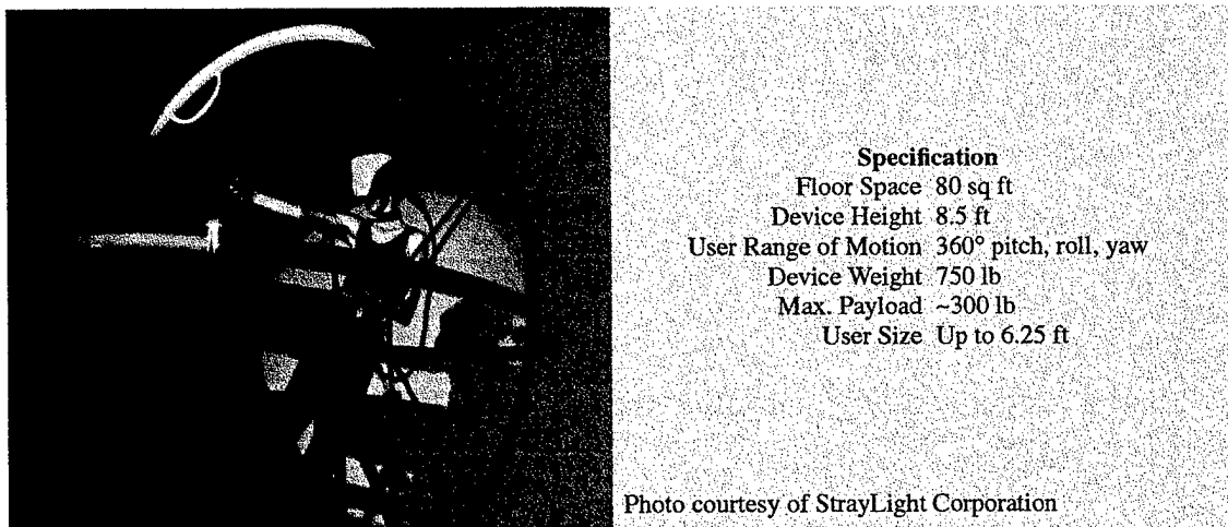
Figure 105. CyberTron
