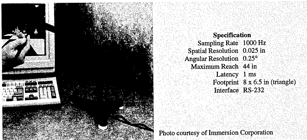
Figure 57. Immersion PROBE-MD
