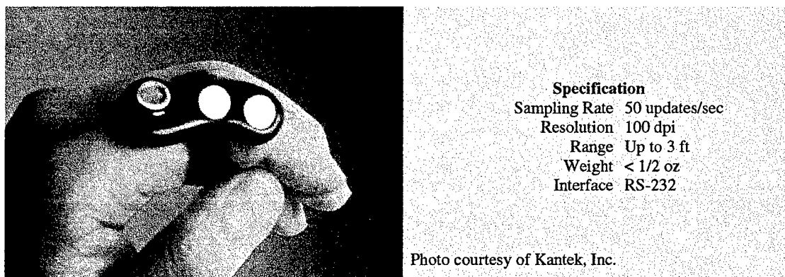
Figure 59. RingMouse
