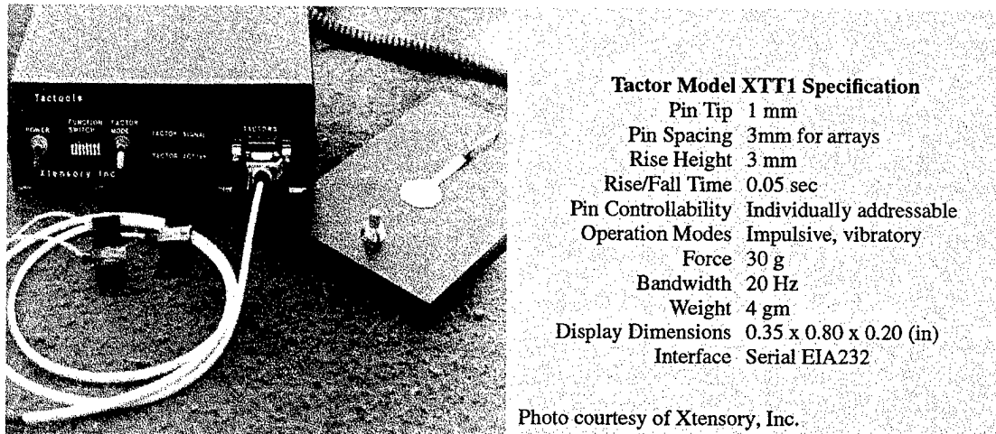
Figure 67. Tactools System
