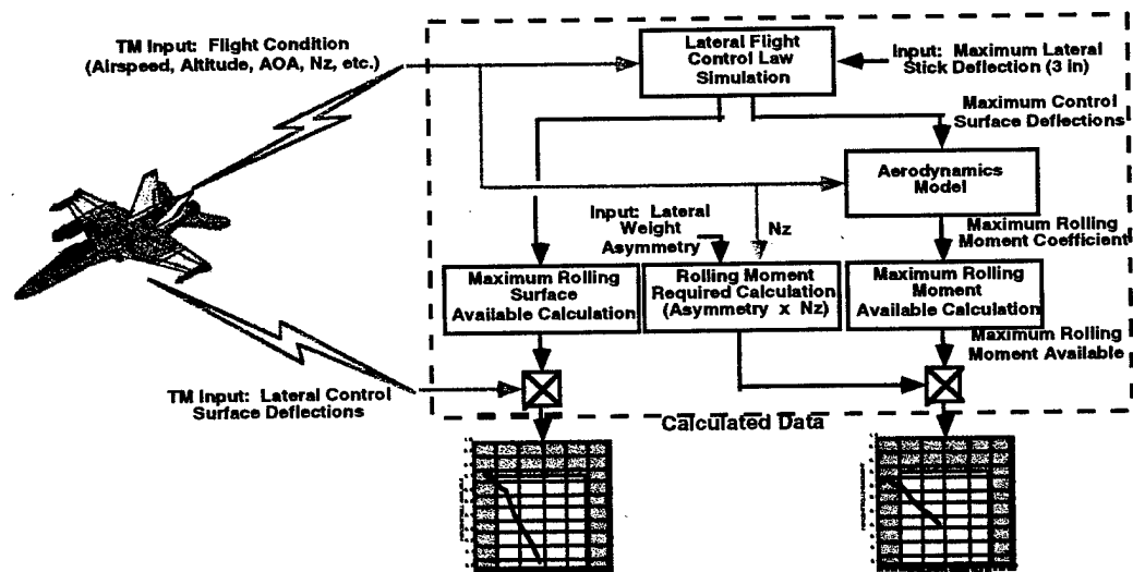
Figure 7 - Real Time Rolling Surface and Moment Calculation Process
