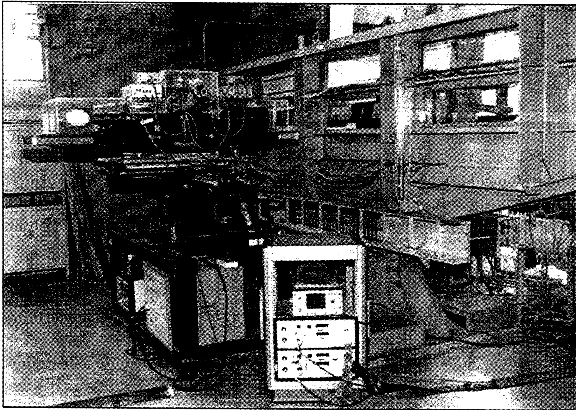
Figure 5. LDV System.
