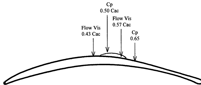
Flow Characteristics at Re=380,000 .
