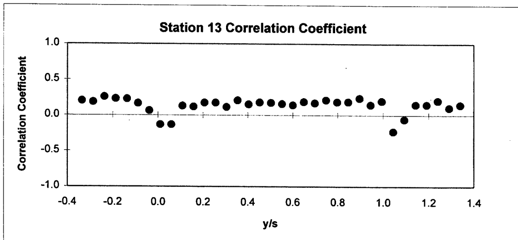
Figure 35. Station 13 Wake Survey Results at Re=210,000 .
