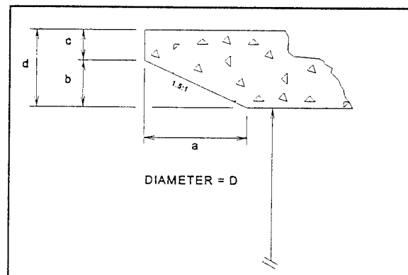
Figure 6.12 Culvert Inlet with Beveled Ring Entrance
