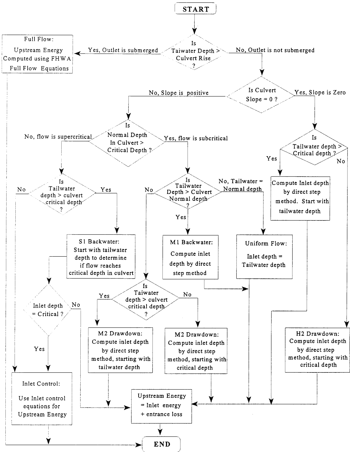
Figure 6.8 Flow Chart for Outlet Control Computations
