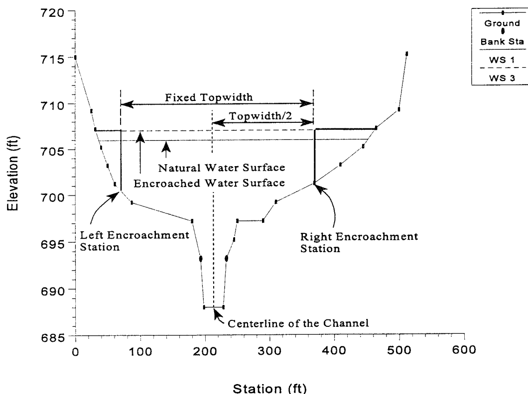
Figure 8.2 Example of Encroachment Method 2
