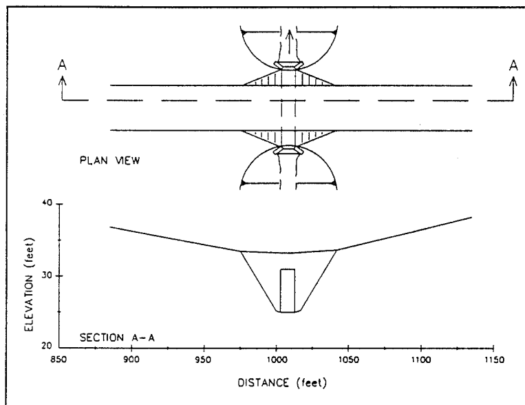
Figure 6.1 Typical Culvert Road Crossing
