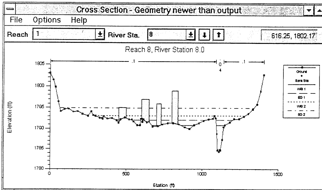
Figure 3.7 Example of a Cross Section With Blocked Obstructions
