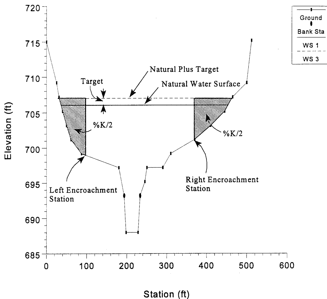
Figure 8.5 Example of Encroachment Method 5
