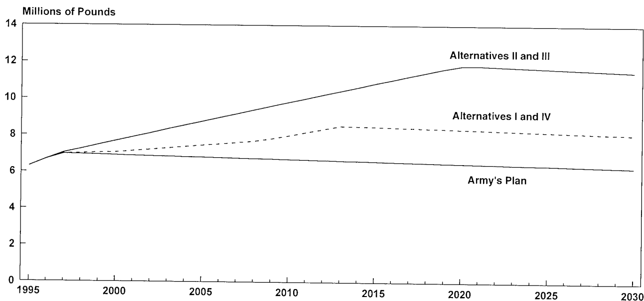
Figure 21. Lift Capacity of the Utility Fleet Under the Army's Plan and Four Alternatives (At 4,000 feet and 95 degrees F)
